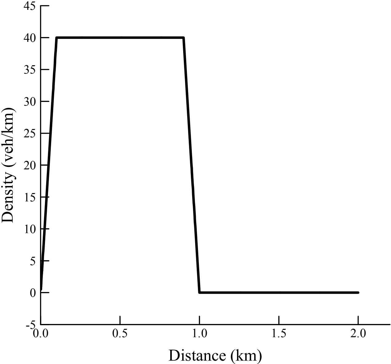
Figure 1 Initial density platoon on the example highway.
