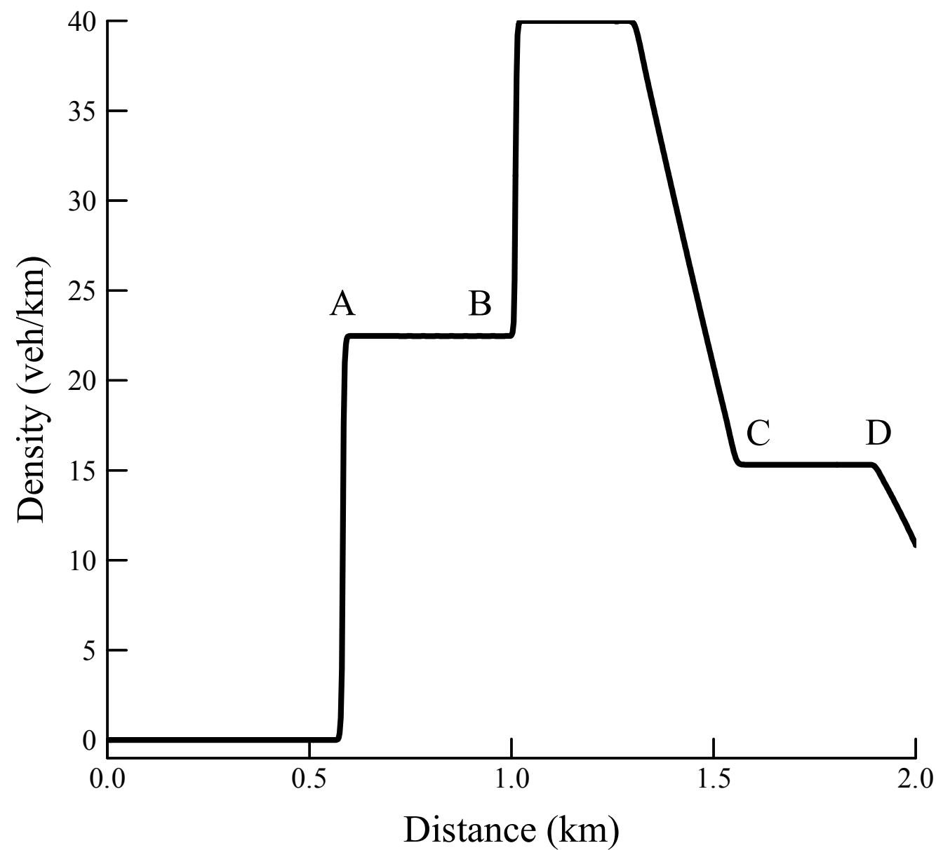
Figure 2 The dispersion of platoon at time t = 0.01 hour.
