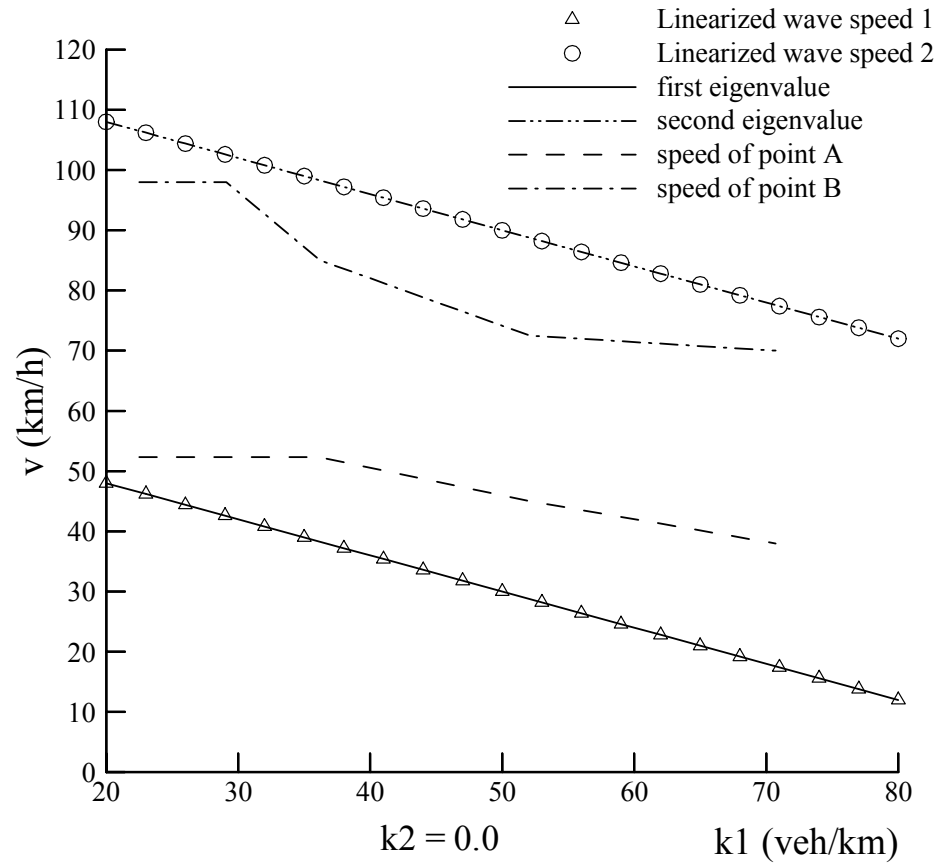
Figure 3 The wave speeds for the 2-class case.
