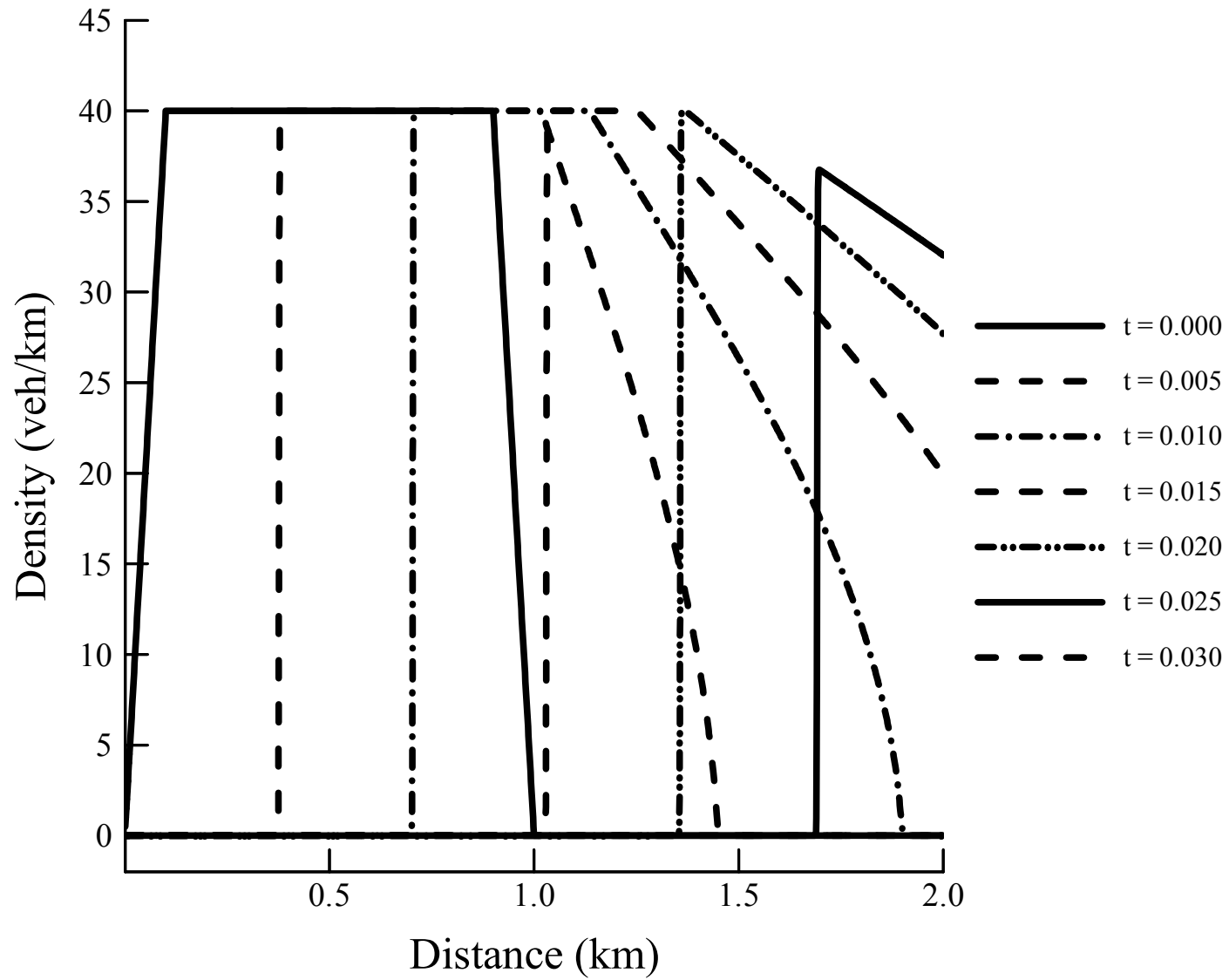
Figure 7 Total density as a function of spatial location, for t = 0, 0.005, 0.010, \dots, 0.030 hours, for the case of 9-class model with identical free speed.
