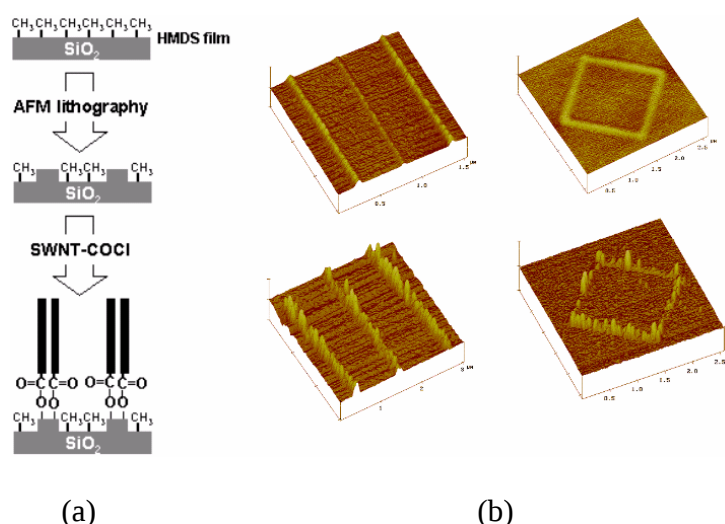
Figure 4 (a) Schematic for selectively attachments of SWNTs on prepatterned surfaces, representative tapping mode AFM images of patterned HAMD SAM (b, top) before and (b, bottom) after reaction with SWNTs.
