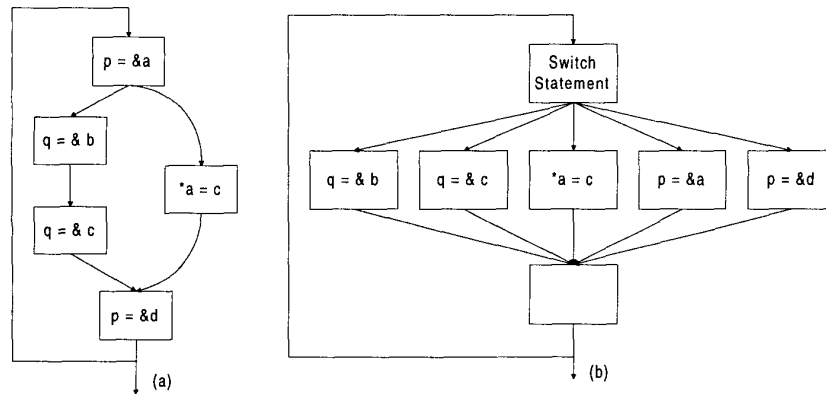
Figure 7: Effect of the degenerate control flow on alias analysis
