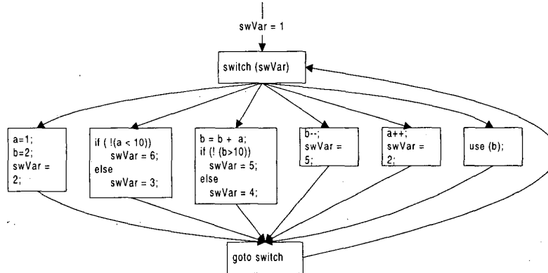
Figure 3: Transforming to indirect control transfers
