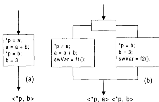
Figure 5: Introducing aliases through pointers
