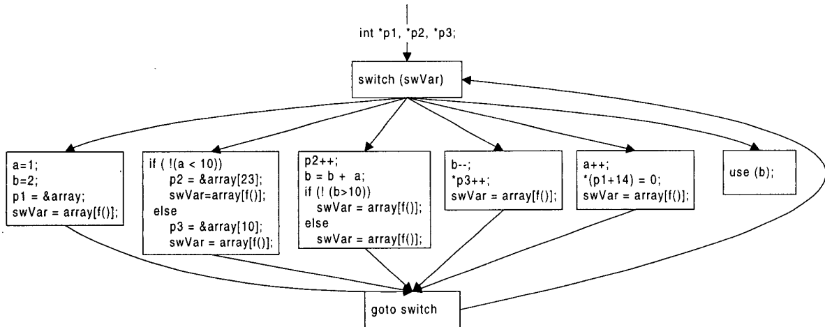
Figure 6: An example transform using pointer manipulation
