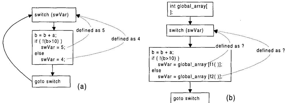
Figure 4: Example illustrating dynamic computation of branch targets
