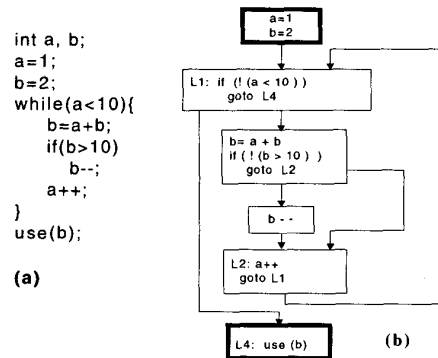
Figure 2: Dismantling high-level constructs
