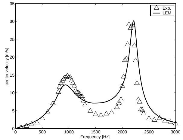
Figure 2: Comparison between the lumped element model and experiment for Case I. 8
