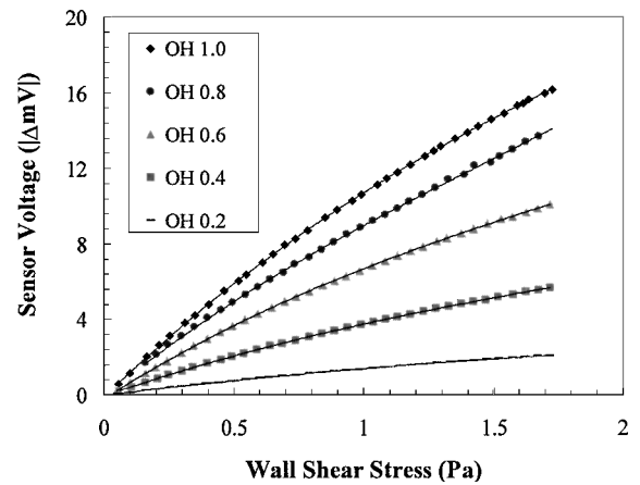
Fig. 4 Static response of the sensor vs shear stress at different overheat ratios, calibrated in the laminar flow channel (third-order polynomial curve fits included).
