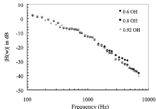
Fig. 8 Plot of the gain factor of the sensor frequency response for a 105-dB SPL sine sweep as a function of overheat ratios.
