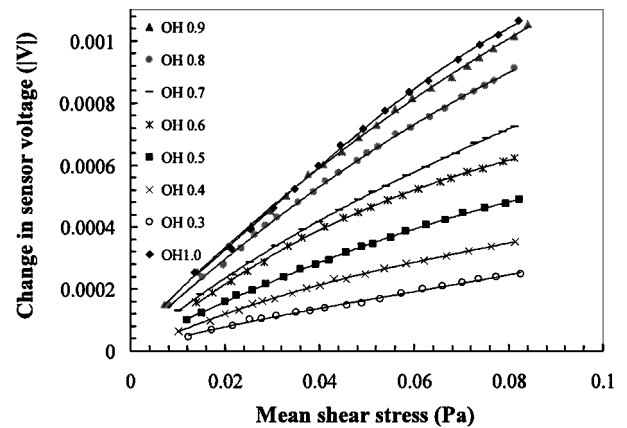
Fig. 5 Static response of the sensor vs shear stress at different overheat ratios, calibrated in the PWT (third-order polynomial curve fits included).
