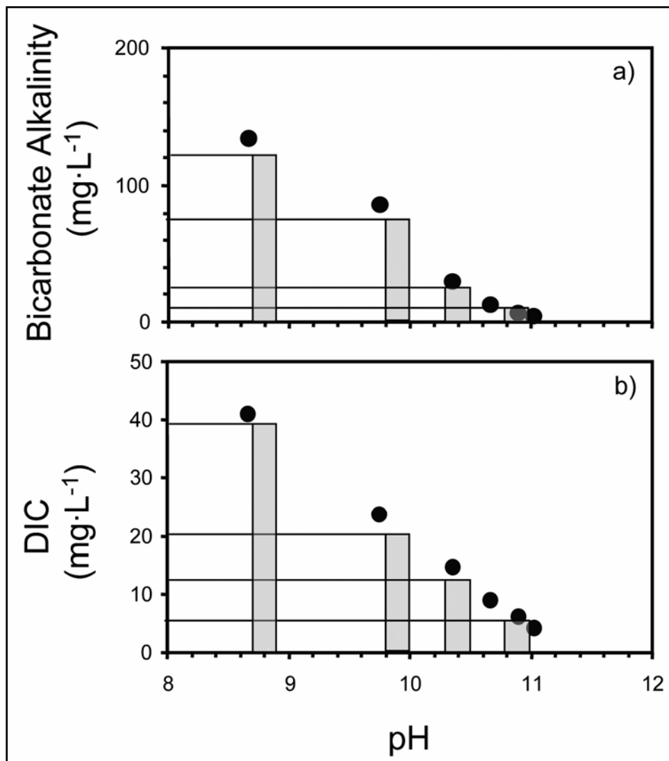
Figure 2. Variations in bicarbonate alkalinity (a) and dissolved inorganic carbon (b) as a function of lime-adjusted increases in pH.
