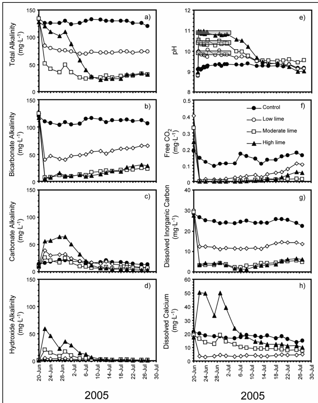
Figure 3. Variations in total alkalinity (a), bicarbonate alkalinity (b), carbonate alkalinity (c), hydroxide alkalinity (d), pH (e), free carbon dioxide ( \text{CO}_2 , f), dissolved inorganic carbon (g), and dissolved calcium (h) in control and experimental mesocosms treated with low, moderate, and high concentrations of lime (as \text{Ca}(\text{OH})_3 ).
