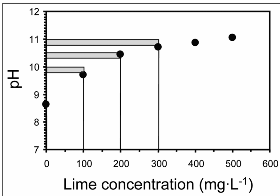
Figure 1. The effects of various concentrations of lime (as \text{Ca(OH)}_2 ) on the pH of mesocosm water. Grey horizontal bars represent the desired pH target ranges and the vertical black lines denote the required concentration of lime.
