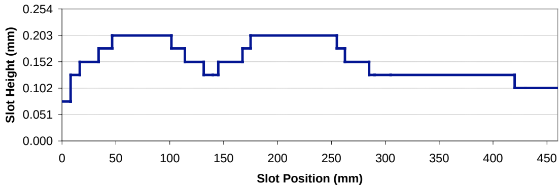
Figure 5.2.2 Spanwise variation in slot height
