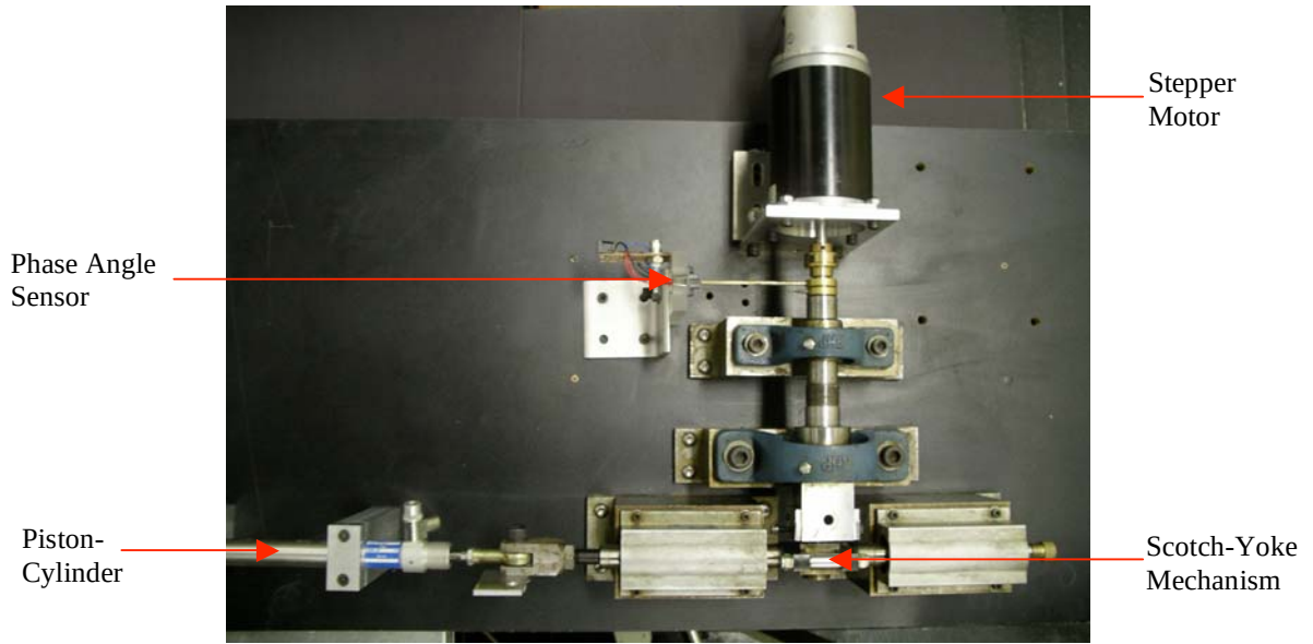
Figure 5.3.1 – Excitation system.
