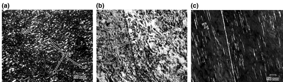
Fig. 3. AF/C-489 150 °C 24 h micrographs (a) CDF image showing \delta' and \theta'/\theta'' englobed with \delta' , b = [0\ 1\ 1]_x g = (1\ 0\ 0)_{\delta'} , (b) BF indicating \theta'/\theta'' and matrix and grain boundary puckering T_1 , b = [1\ 1\ 0]_x , (c) CDF micrograph showing matrix and grain boundary puckering T_1 , b = [1\ 1\ 0]_x g = \frac{1}{2}(1\ 1\ 1)_x .
