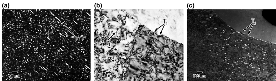
Fig. 2. AF/C-458 150 °C 24 h micrographs (a) CDF image showing \delta' and \theta'/\theta'' englobed with \delta' , b = [0\ 1\ 1]_x g = (1\ 0\ 0)_{\delta'} , (b) BF indicating \theta'/\theta'' and matrix and grain boundary puckering T_1 , b = [1\ 1\ 0]_x , (c) CDF micrograph showing matrix and grain boundary puckering T_1 , b = [1\ 1\ 0]_x g = \frac{1}{2}(1\ 1\ 1)_x .
