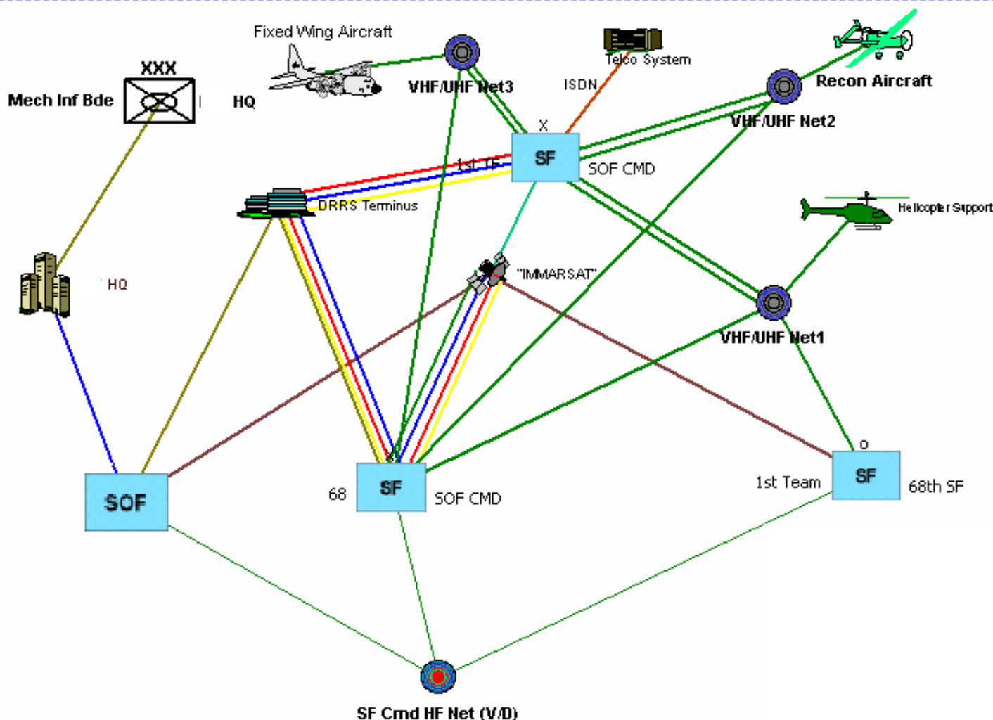
SOF System Architecture
