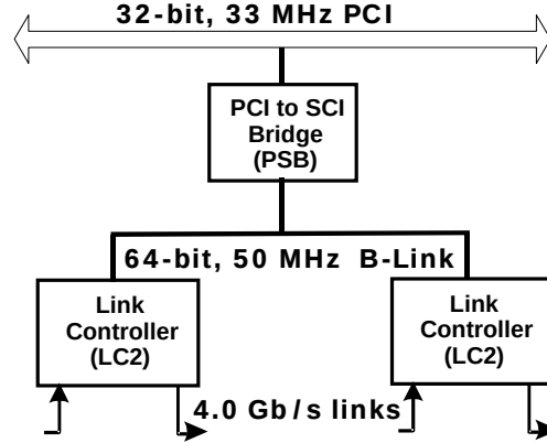
Fig. 4. Architectural components of a Wulfskit SCI NIC.
