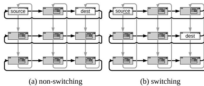
Fig. 10. Torus test configurations.
