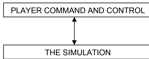
Figure 2: Wargame Structure
