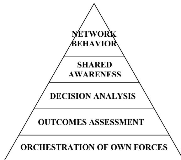
Figure 1: Gaming Dimensions
