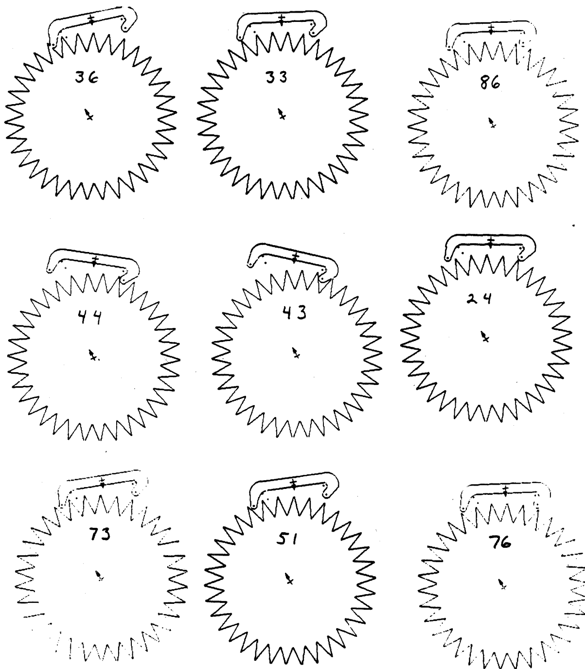
Figure 9.13: Sample configurations for the escapement's places
