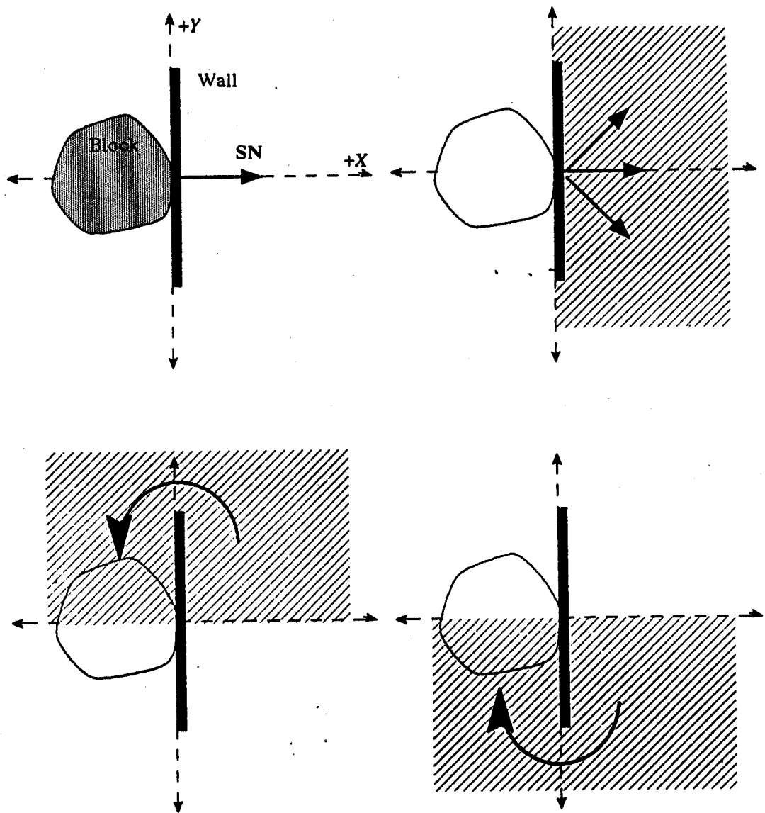
Figure 3.1: Constraints imposed by surface contact
