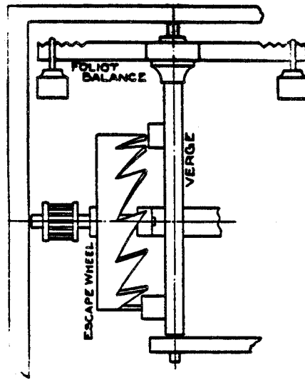
Figure 11.1: Verge escapement
