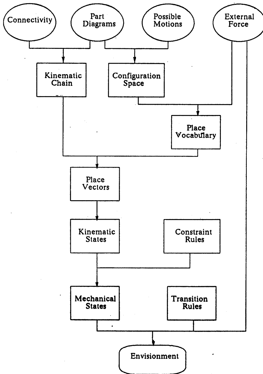
Figure 1.1: Information flow of Qualitative Mechanics
