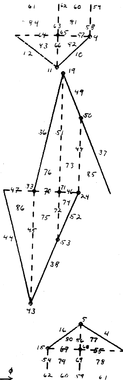
Figure 9.10: Place vocabulary for scape wheel and pallets
