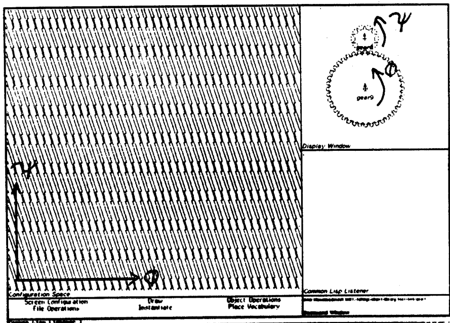
Figure 9.7: The configuration space for gears 9 and 8
