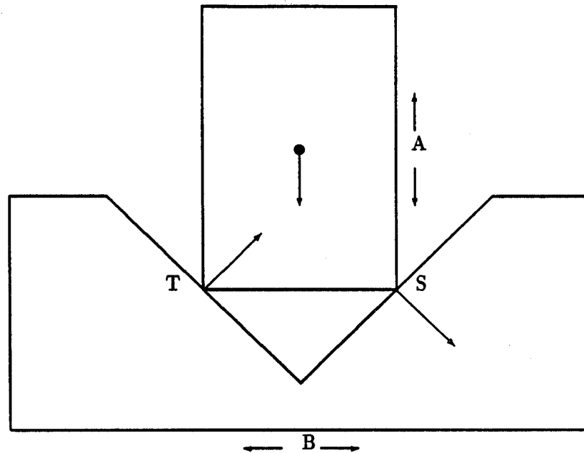
Figure 5.2: Force feedback example
