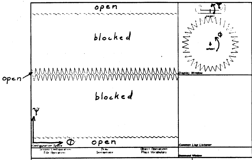
Figure 9.2: The configuration space for scape wheel and pallets
