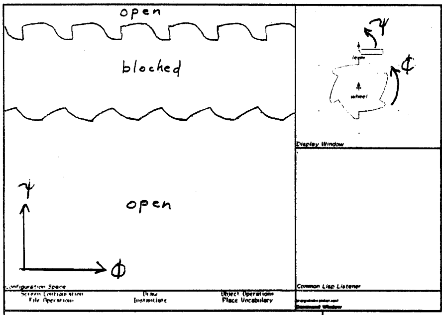
Figure 9.9: The configuration space for ratchet and pawl
