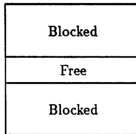
Figure 8.3: Configuration space for a piston in a cylinder
