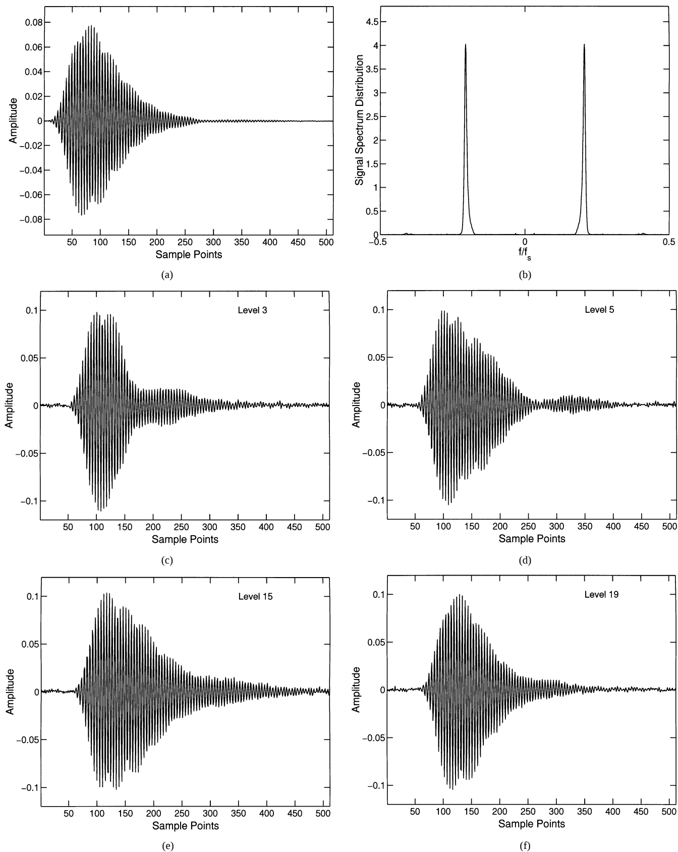
Fig. 5. Recorded waveforms in the real experiment. (a) Transmitted waveform. (b) Discrete Fourier transform of signal in (a). (c) Received signal at level 3. (d) Received signal at level 5. (e) Received signal at level 15. (f) Received signal at level 19.
