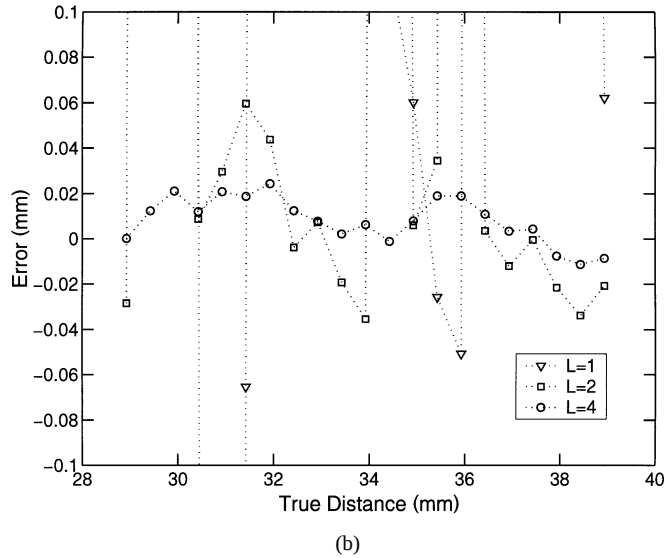
Fig. 7. Stationary level measurement results obtained by applying the multi-PEARS algorithm to the measured signal with the different choices of L . The ranging distance covers from 29 to 39 mm. The distance between two consecutive levels is 0.5 mm. (a) Measurement results versus the true distance obtained by traverse. (b) Measurement errors.
