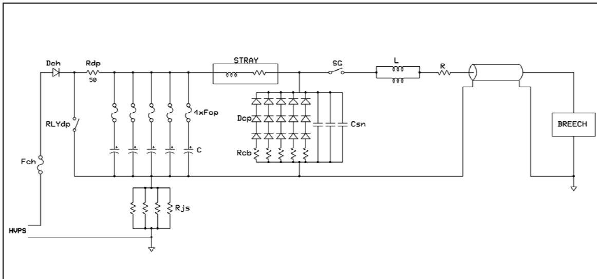
Figure 2. Module schematic.
