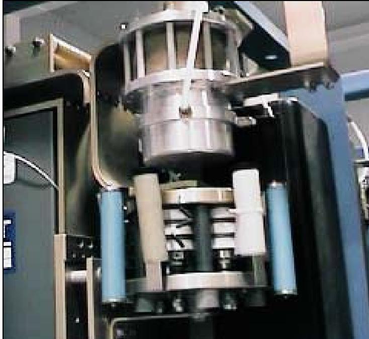
Figure 4. Crowbar diodes (lower image) and output switch, ST-300 (upper image).
