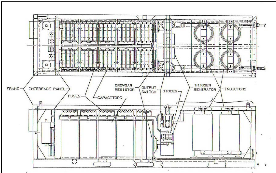
Figure 3. Component layout for one rack ( 2 \times 250 kJ).
