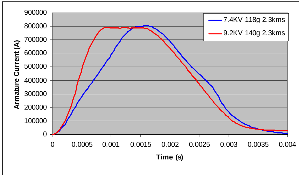
Figure 14. Comparison of pulse shapes for 7.4 and 9.2 kV.
