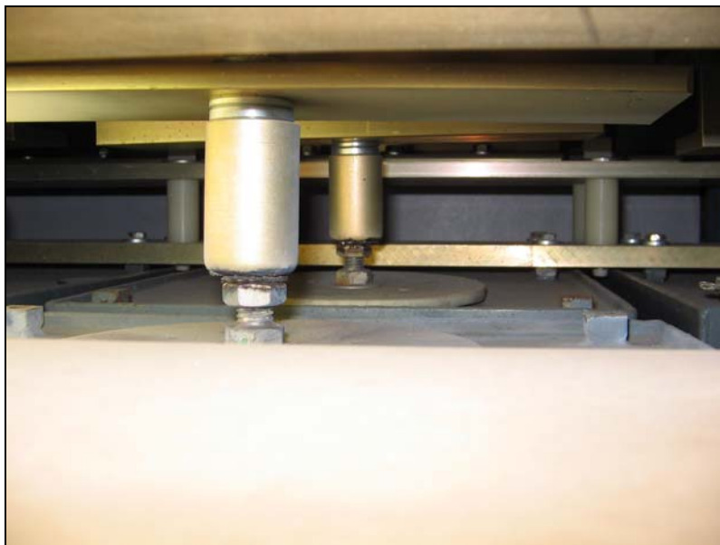
Figure 12. Arc damage at the center post terminals of capacitors.
