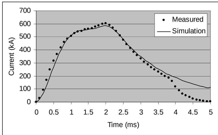
Figure 20. Comparison between measured and simulated currents at 6 kV (mCTL shot 370).
