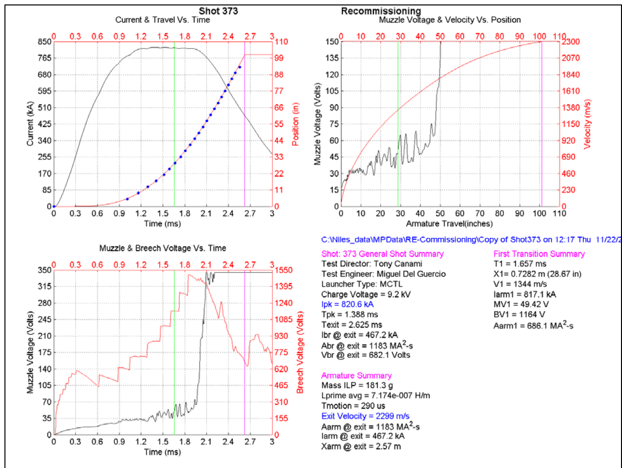
Figure 21. Data summary page from commissioning shot at 9.2 kV (mCTL 373).
