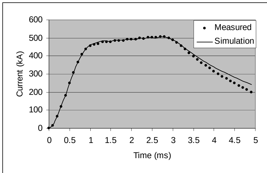
Figure 18. Comparison between data and simulation for sequential discharge test (18 modules).
