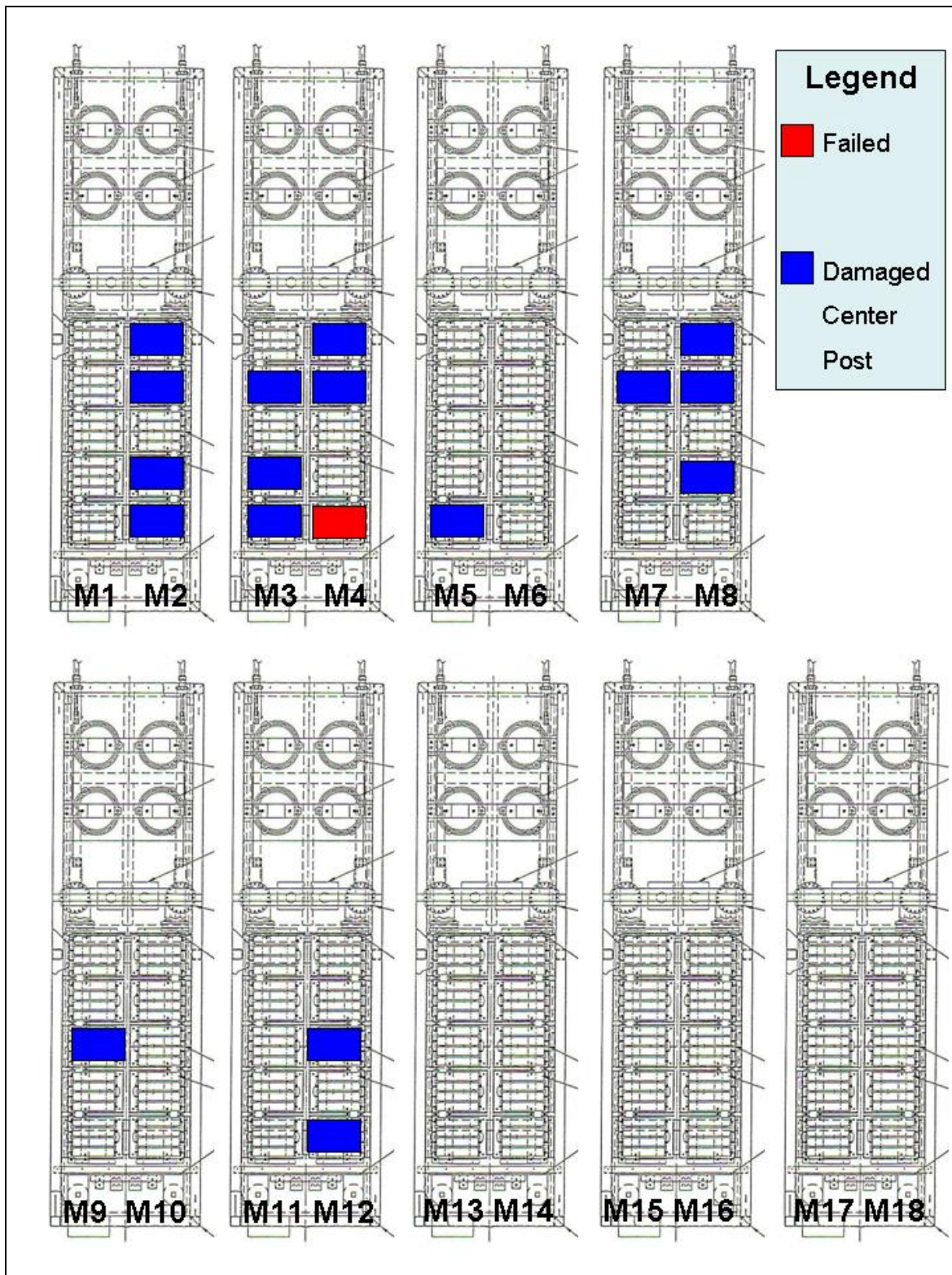
Figure 13. Schematic illustration of affected capacitors.
