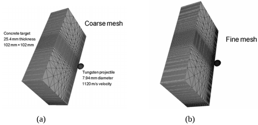
Fig. 5. Ballistic problem: coarse mesh (a) and fine mesh (b).
