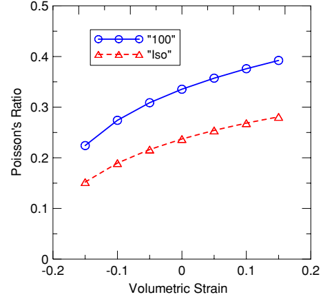
Figure 7. Poisson's ratio in isotropic silicon and in the (100)-direction of cubic silicon as functions of the applied volumetric strain in strained silicon.
