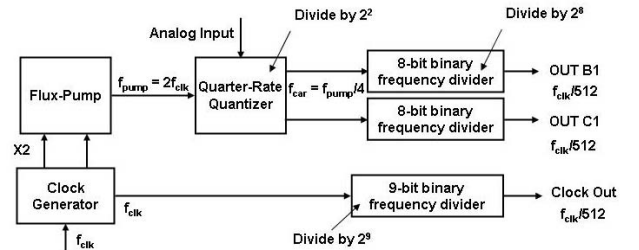
Fig. 9. Block diagram of a chip for high frequency testing of the quarter-rate quantizer.
