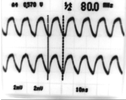
Fig. 10. Oscilloscope traces showing high frequency operation of the quarter-rate quantizer. External clock is applied at a frequency of 40.96 GHz, implying an input frequency of 81.92 GHz to the quantizer. Bottom trace represents the decimated clock output whereas the top trace represents one of the decimated data outputs.
