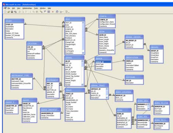
Structure and relationships of BOP database
