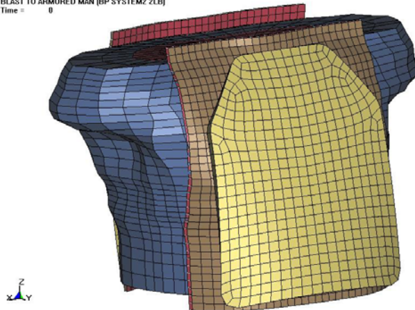
Human FEM with plate and Kevlar
