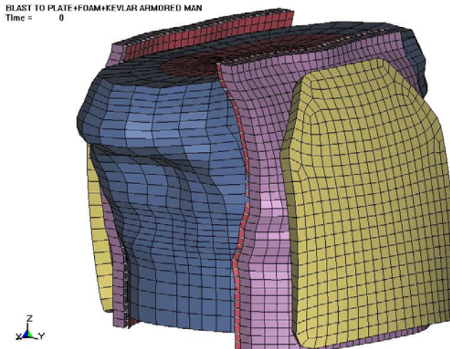
Human FEM with plate, foam and Kevlar
