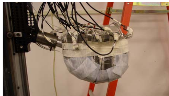
Fully instrumented headform
