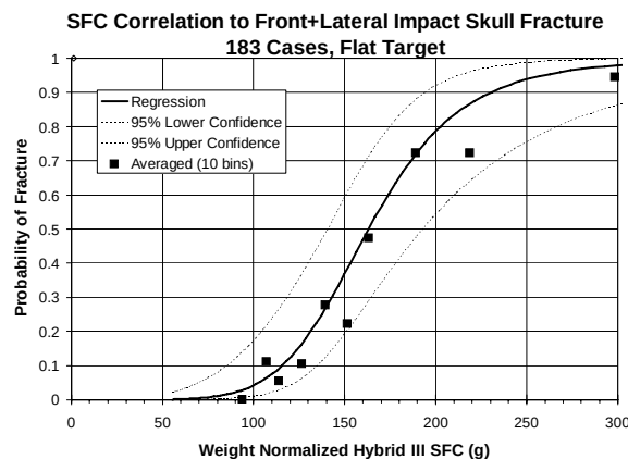
SFC correlation with fracture data
