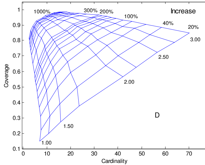
Figure 17: Surface Plot Obtained from Confidence Set Estimator Showing Estimated Relationships Between Set Cardinality, Coverage, Percent Increase from v_0 , and Reference Value D. \alpha = 1 , v_0 = 1 , \tau = 50 , and N = 10,000 .
