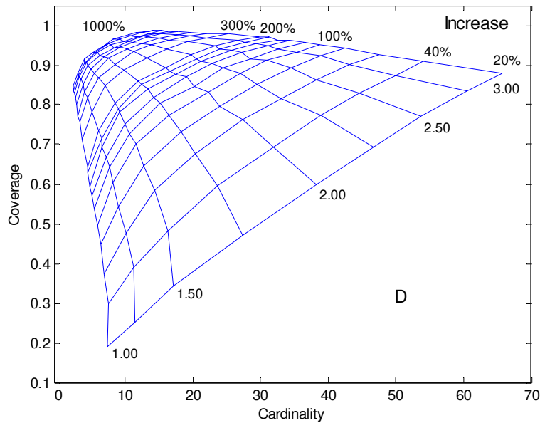
Figure 18: Surface Plot Obtained from Confidence Set Estimator Showing Estimated Relationships Between Set Cardinality, Coverage, Percent Increase from v_0 , and Reference Value D. \alpha = 1 , v_0 = 5 , \tau = 50 , and N = 10,000 .
