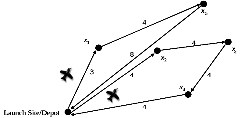
Figure 1. Example vehicle routing problem network.
