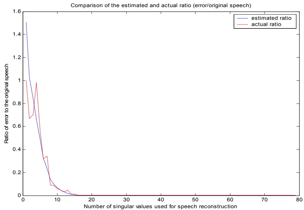
Figure 2.22: Comparing the actual error ratio to the estimated error ratio for a specific frame of speech. Note: E_{\text{error}}/E_{\text{sr}} (blue), A_{\text{error}}/A_{\text{sr}} (red)
