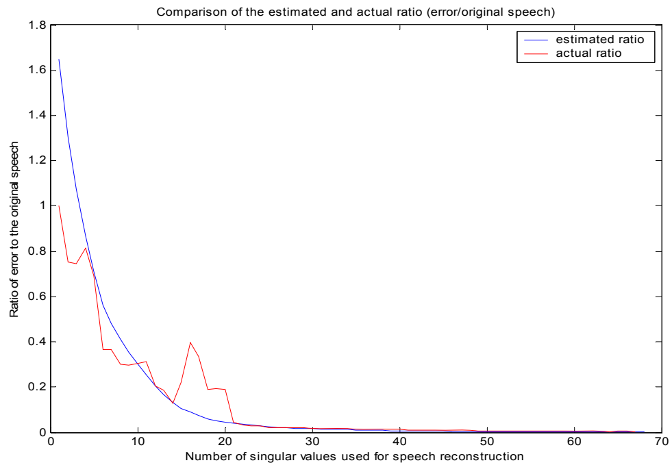
Figure 2.21: Comparing the actual error ratio to the estimated error ratio for a specific frame of speech. Note: E_{\text{error}}/E_{\text{sr}} (blue), A_{\text{error}}/A_{\text{sr}} (red)
