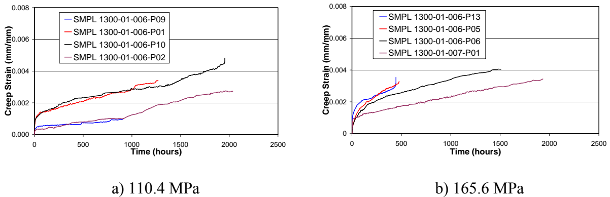
Figure 4. Long-term Creep Curves
