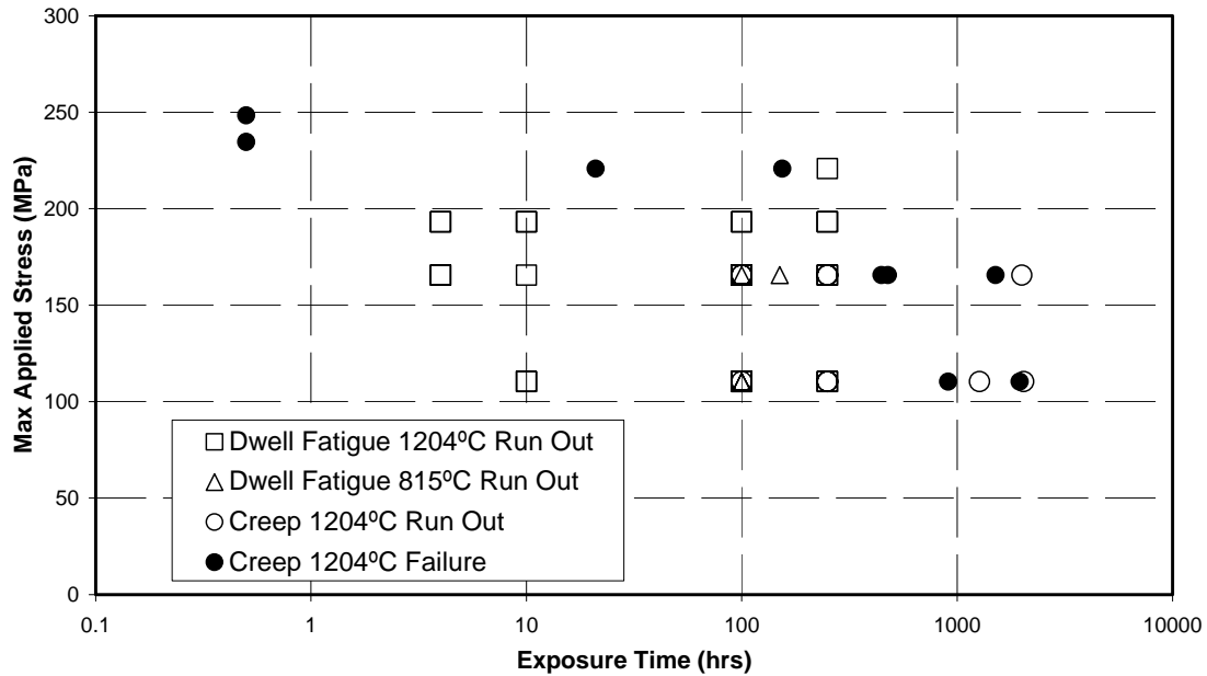
Figure 3. Creep and Dwell Fatigue Testing Summary
