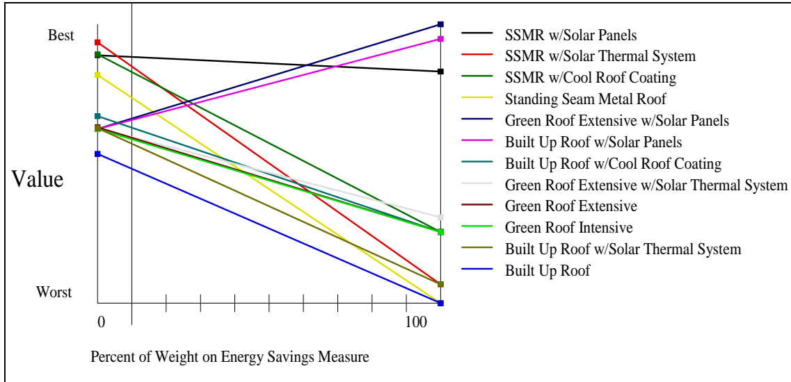
Figure 4.19. Sensitivity Analysis of Environmental Objective at West AFB.
