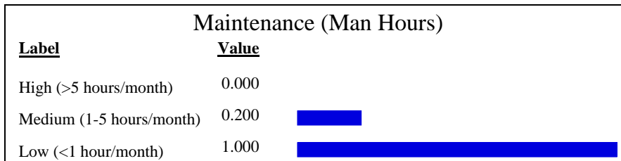
Figure A10. SDVF for Southeast AFB Maintenance Evaluation Measure. This a discrete, categorical function.
