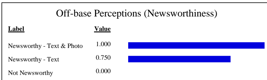
Figure A11. SDVF for Southeast AFB Off-base Perceptions Evaluation Measure. This a discrete, categorical function.
