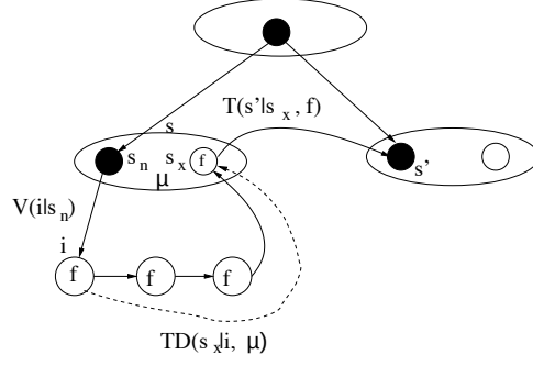
Figure 18: The dashed arrow is the discounted transition probability for reaching state S_x from state i . The solid arrows are simply the transition probabilities for the forward action.
