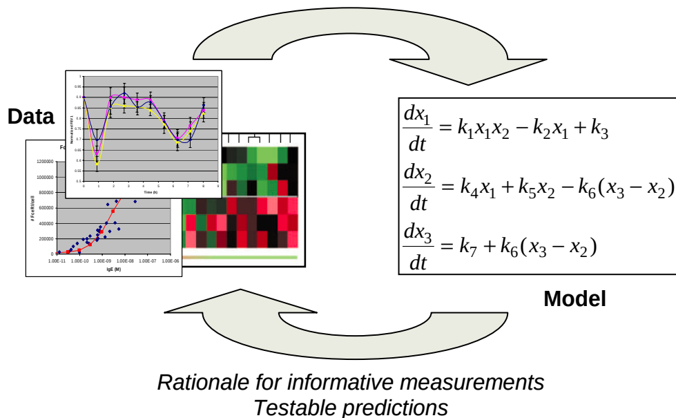
Figure 4.3. With the purpose of increasing understanding of a biological system function, one needs a set of data to develop the first model. That first model can then be simulated or analyzed to pinpoint uncertainties that are important to the system and then recommend a new set of experiments to measure relevant quantities to reduce those uncertainties. The new data can be used to revise the model. The model at various stages of iteration can also be used to test hypotheses about the system's function or means of modulating that function, and interesting predictions from those tests can then also be verified (or refuted) experimentally.
