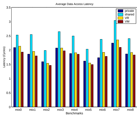
Figure 17. Access latencies of multi-programmed workloads. Configuration 3: 16+16/512/24FO4.
