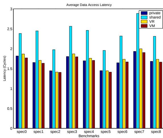
Figure 18. Access latencies of multi-programmed workloads. Configuration 4: 16+16/1024/24FO4.
