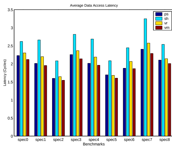
Figure 16. Access latencies of multi-programmed workloads. Configuration 2: 16+16/256/24FO4.
