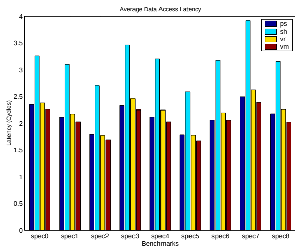
Figure 15. Access latencies of multi-programmed workloads. Configuration 1: 8+8/256/16FO4.
