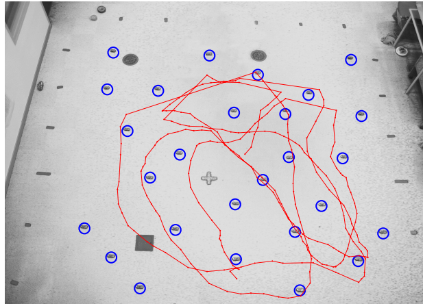
Figure 6.4: Sensor locations and mobile trajectory for a medium size network. Circles outline each of the 27 sensor nodes. Markers on the trajectory depict the location of events. 250 of the 1500 events are shown, with consecutive events connected by a line. The mobile was offset from the ground plane and could pass over nodes. To generate this figure, a homography that accounts for the camera transformation was used to project real-world coordinates to image coordinates.
