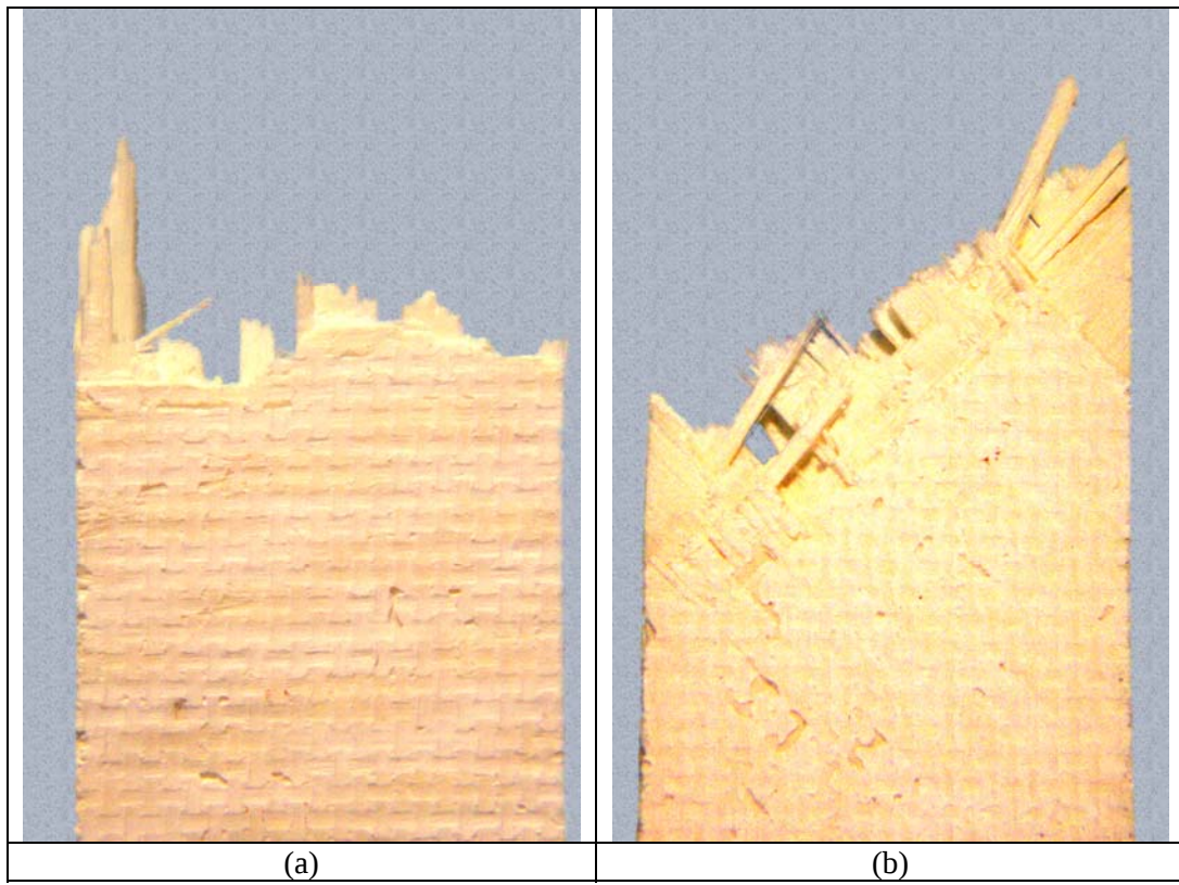
Figure 6. Fracture surface of tensile tested Nextel TM 720/AS-0 at 1100°C (a) 0°/90°, (b) ±45°.
