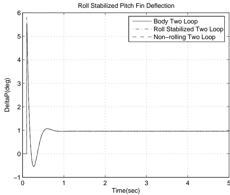
Figure 19. Roll Stabilized Pitch Fin Deflection
