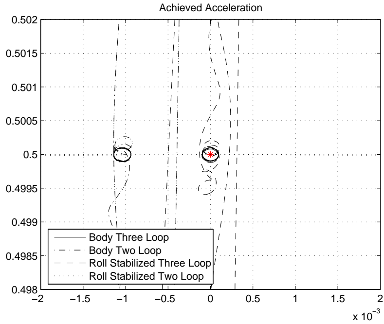
Figure 16. Acieved Acceleration
