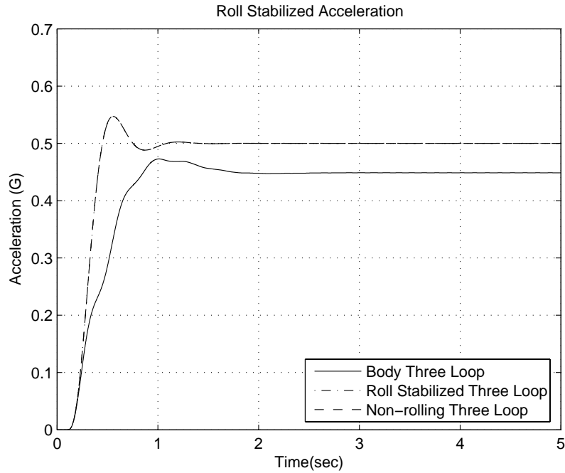
Figure 18. Roll Stabilized Acceleration
