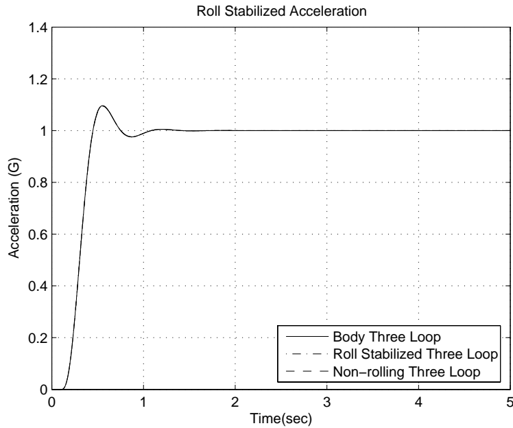
Figure 3. Roll Stabilized Acceleration
