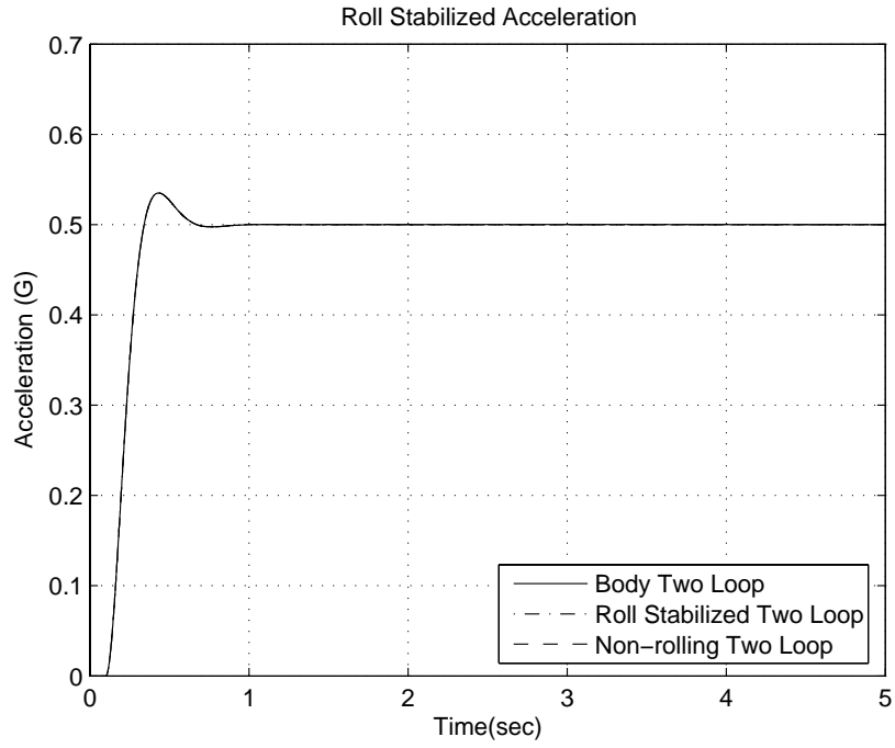
Figure 20. Roll Stabilized Acceleration
