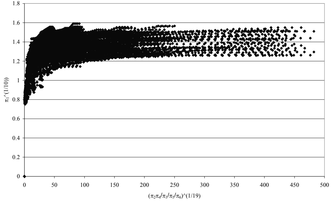
Figure 6.4 Lateral \Pi Theorem Analysis
