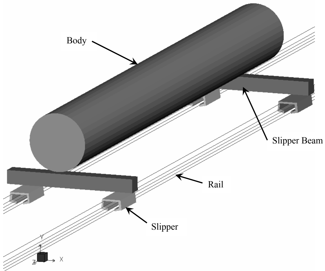
Figure 5.1 Reduced Complexity Model Depiction
