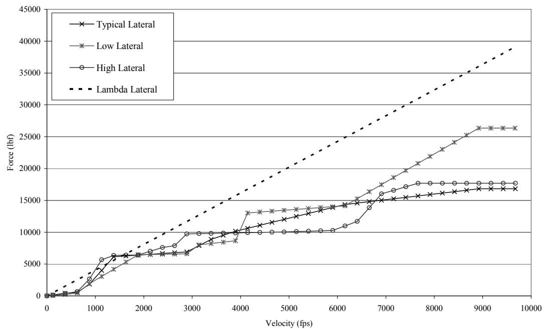
Figure 5.8 Initial Parameter Variation Lateral Force Results: Mass
