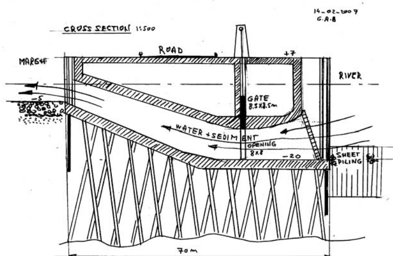
Figure 82 Cross section of a sediment and river water diversion structure.
