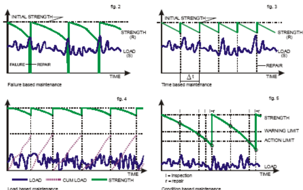
Figure 87 Maintenance concepts
