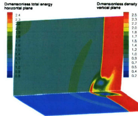
Fig. 15 Total energy and density contours for real gas model
