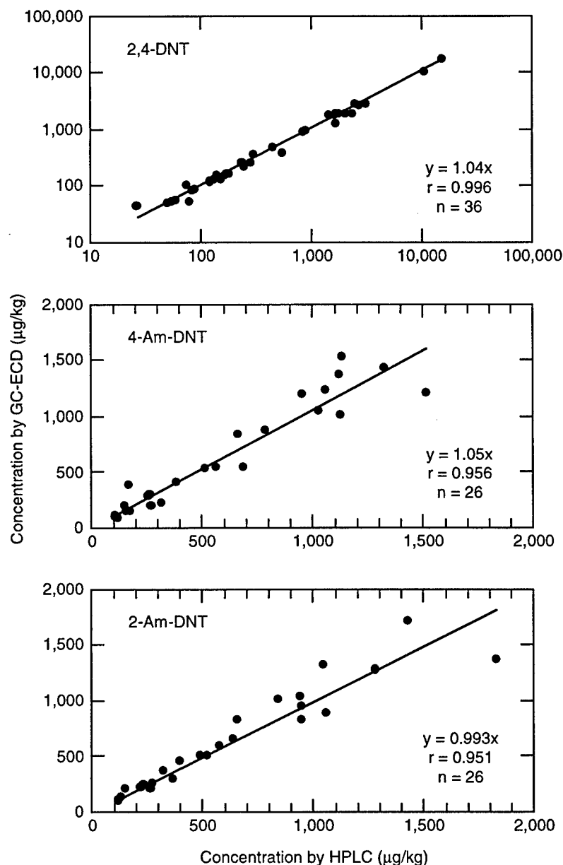
Figure 7. Correlation analysis of GC-ECD concentration ( \mu\text{g/kg} ) estimates with those from HPLC-UV analysis using splits of the same acetonitrile extracts from soils collected from an experimental minefield.
