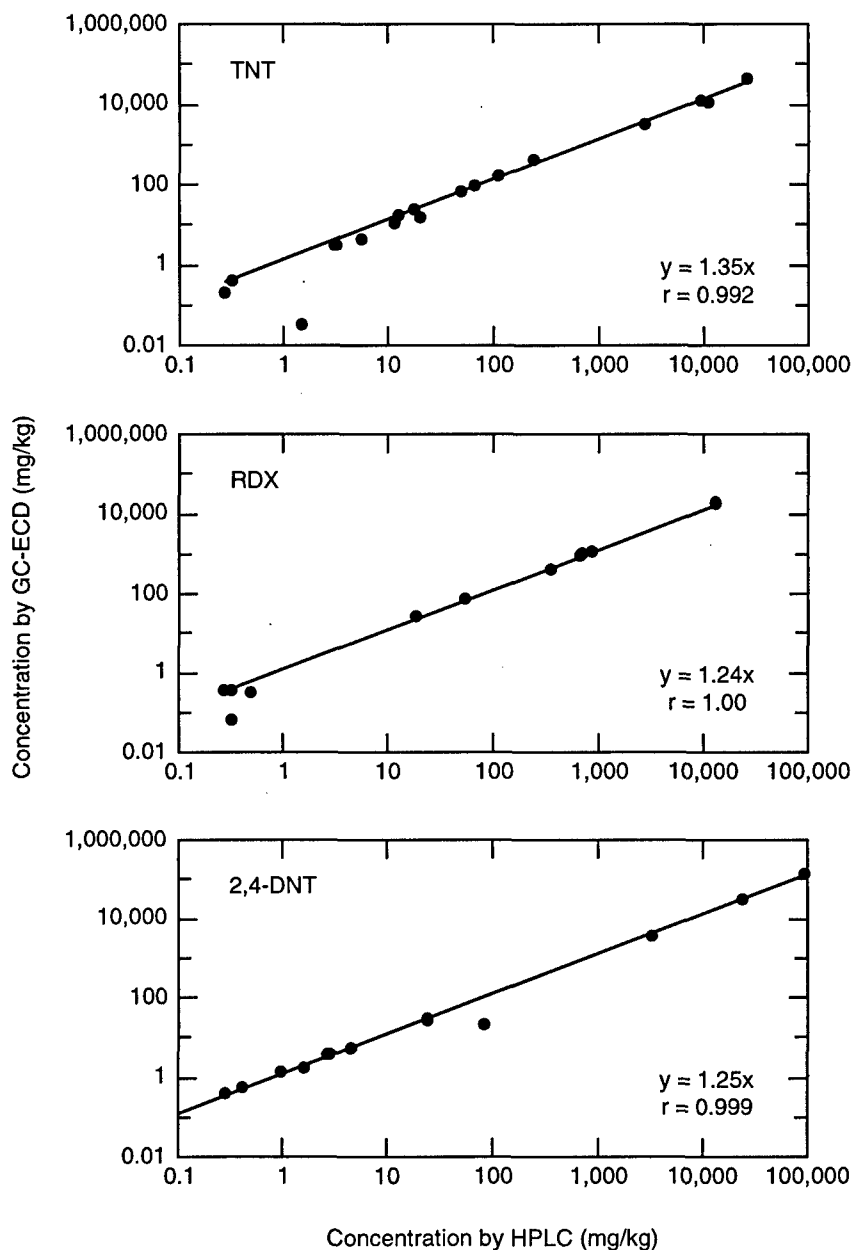
Figure 1. Correlation analysis of GC-ECD concentration (mg/kg) estimates with those from HPLC-UV analysis using splits of the same acetonitrile extract (2 g soil:10 mL acetonitrile) from archived soils.
