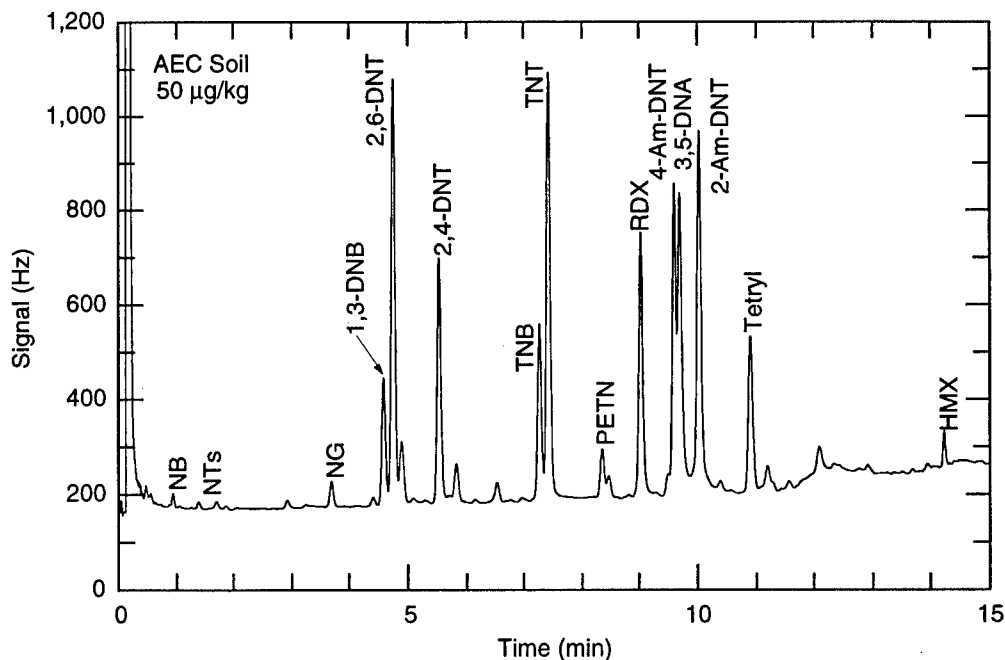
c) AEC soil, 50 \mu\text{g}/\text{kg} .
