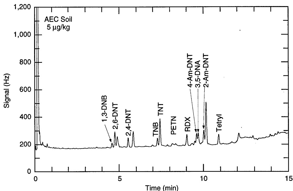
b) AEC soil, 5 \mu\text{g}/\text{kg} .
