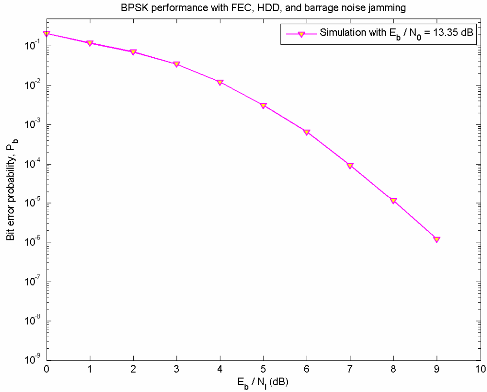
Figure 22. Performance for BPSK with r=1/2 , v=3 convolutional source coding, HDD, and barrage noise jamming.
