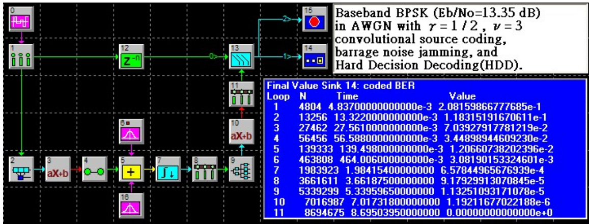
Figure 21. The simulation of baseband BPSK in AWGN with r=1/2 , v=3 convolutional source coding, HDD, and barrage noise jamming.
