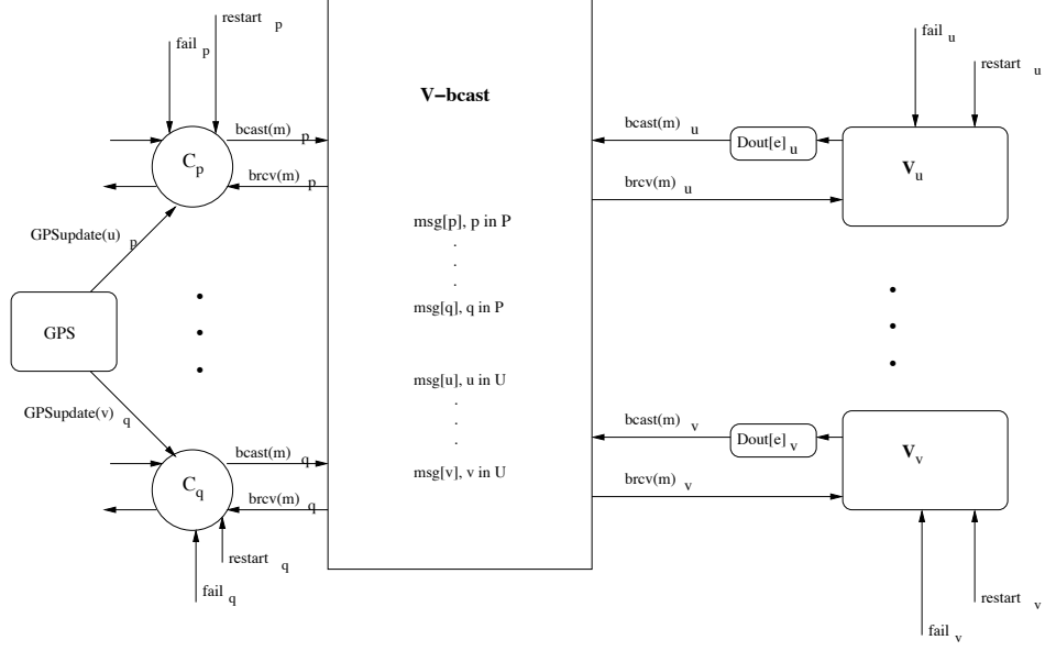
Fig. 3. Virtual Stationary Automata abstraction. VSAs and clients communicate using the V-bcast service. VSA bcasts may be delayed in Dout buffers.
