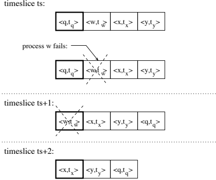
Fig. 5. Handling failures in the guards vector. Process w fails in timeslice ts. In timeslice ts+1, after the vector rotates, w is supposed to be leader. Other guards do not receive a hand-off from w and remove w from the vector at the beginning of timeslice ts+2.
