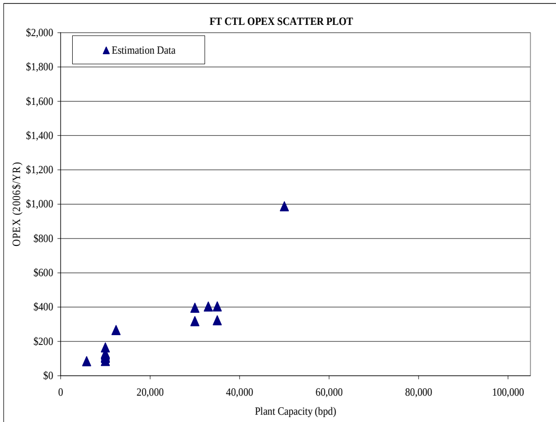
Figure 14 FT CTL OPEX Scatter Plot of Estimation Data
