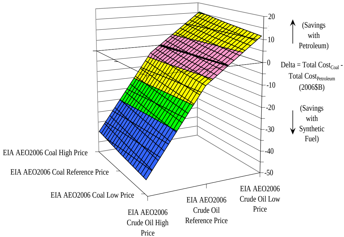
Figure 37 Decision Space with Third Dimension of Delta Value
