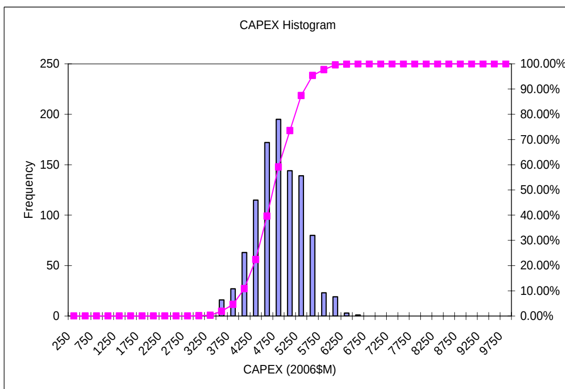
Figure 16 MC Simulation Histogram CAPEX Range for 60,000 bpd Plant
