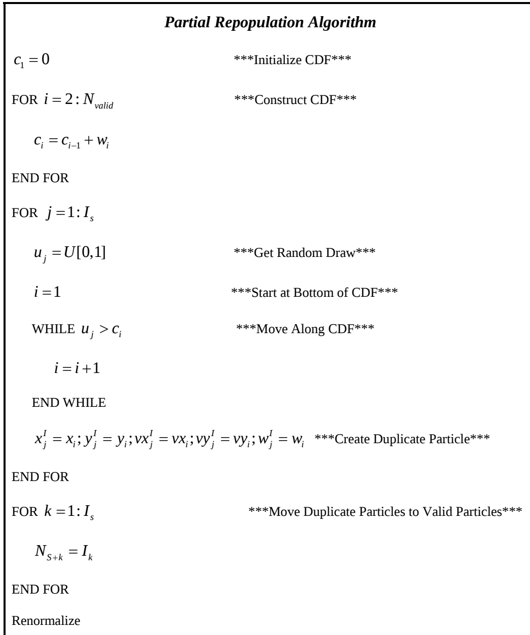
Figure 32. Partial Repopulation Algorithm
