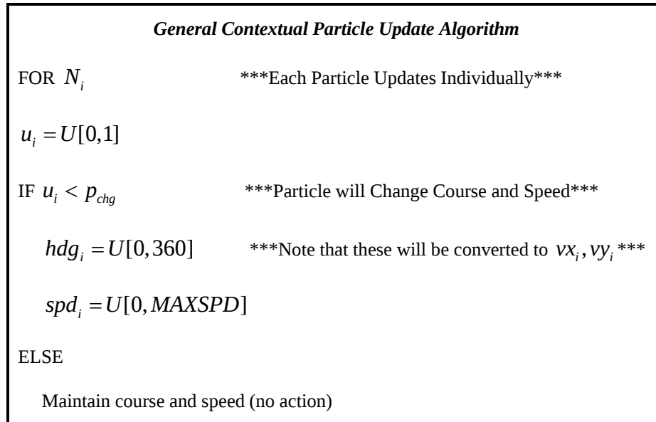
Figure 48. General Contextual Particle Update Algorithm
