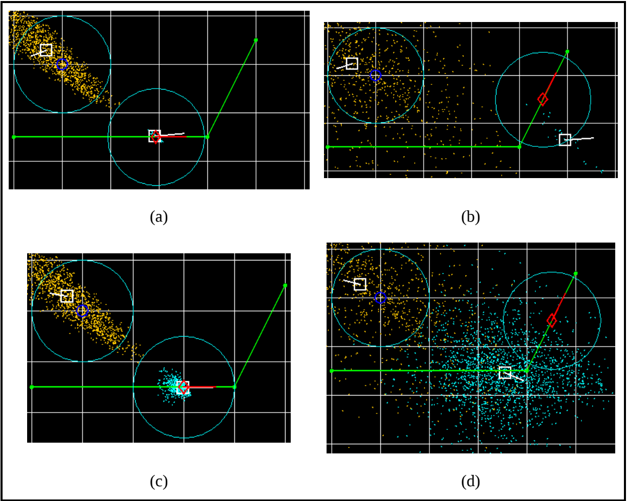
Figure 49. Difference between Naïve and General Contextual Particle Tracking
