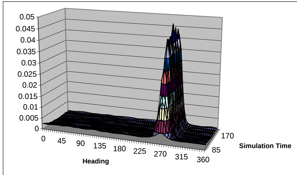
Figure 72. Time-Lapsed Parzen-Windows Approximation of Transitioning Contextual Particle Filter Heading Density (Window Width 7.2)
