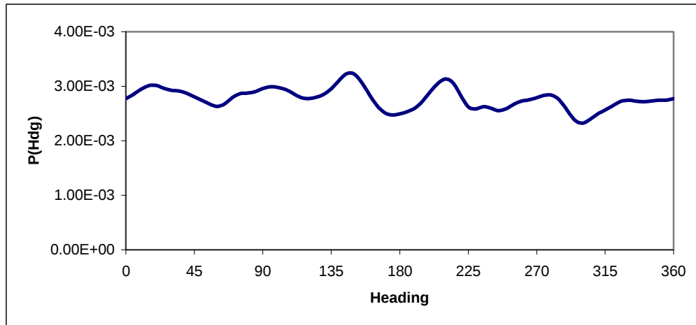
Figure 26. Parzen-Windows Approximation of Initial Detection Distribution Heading Density (Window Width 7.2)
