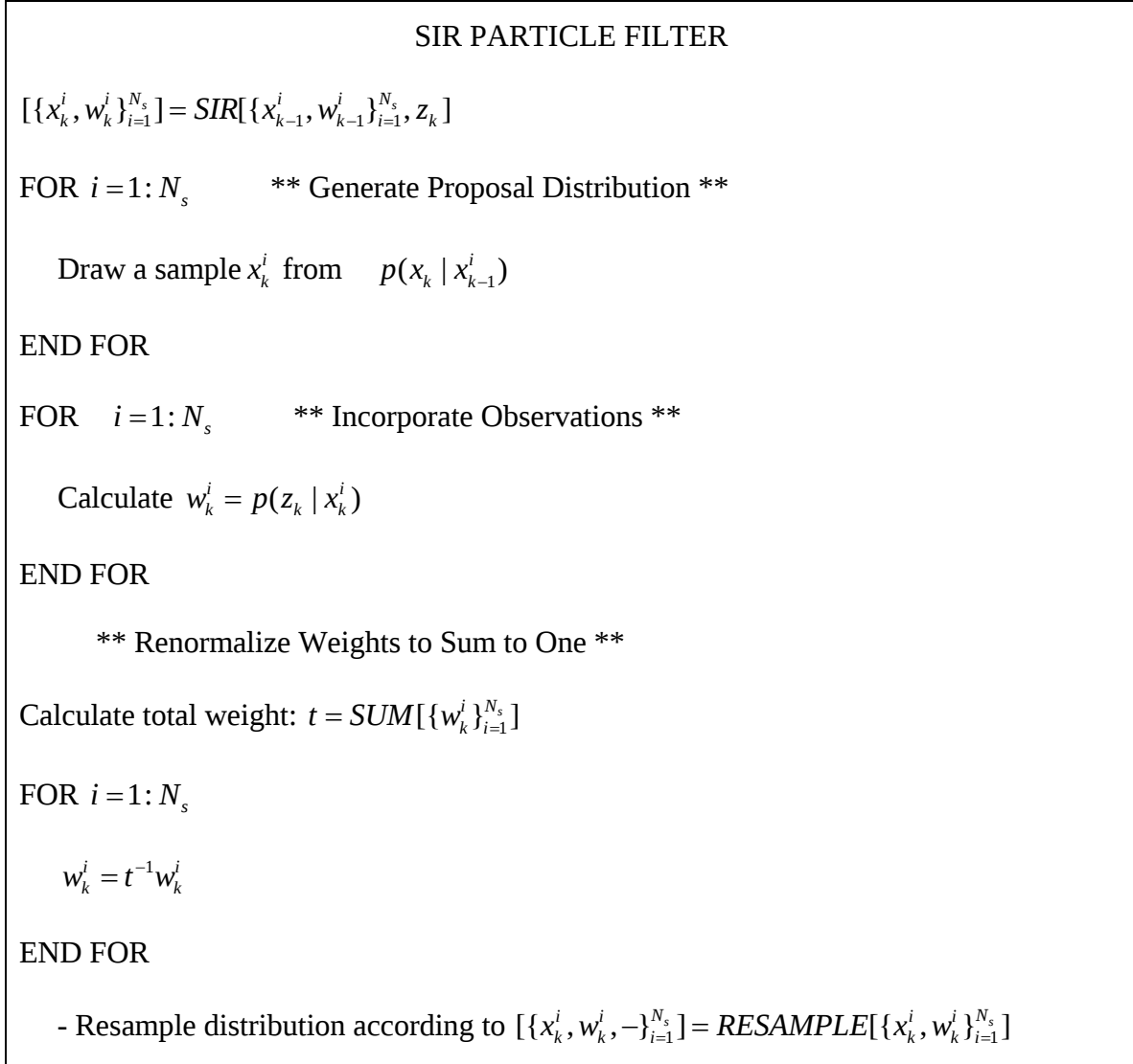
Figure 8. Sampling Importance Resampling Filter Algorithm (After Arulampalam et al. , 2001)
