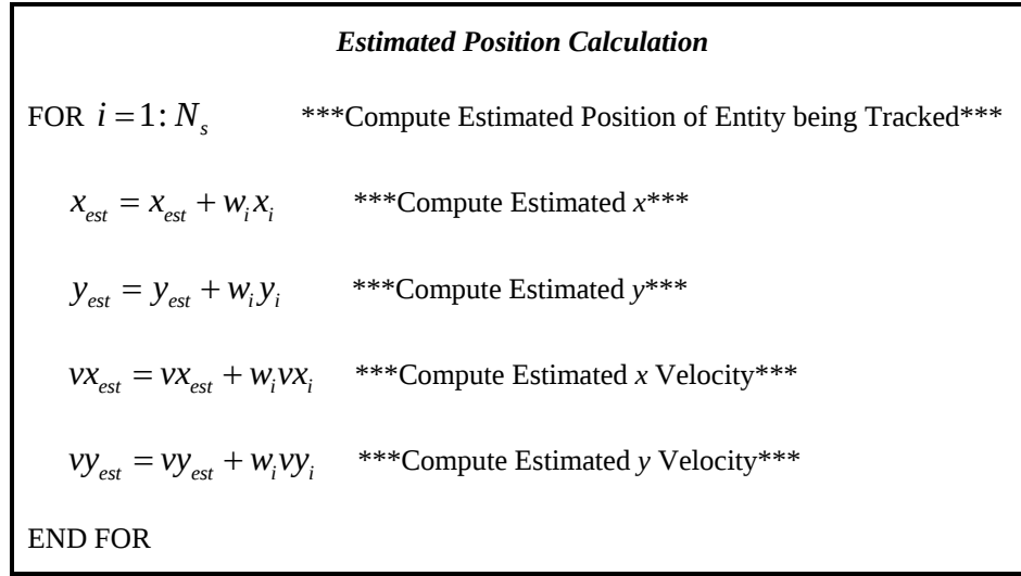
Figure 29. Computing an Estimated Position from a Particle Track
