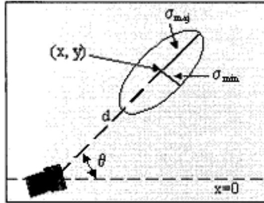
Figure 2. Distribution Parameter Definitions (From Stroup et al. , 2000)
