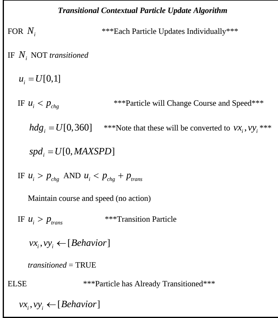
Figure 50. Transitional Contextual Particle Update Algorithm
