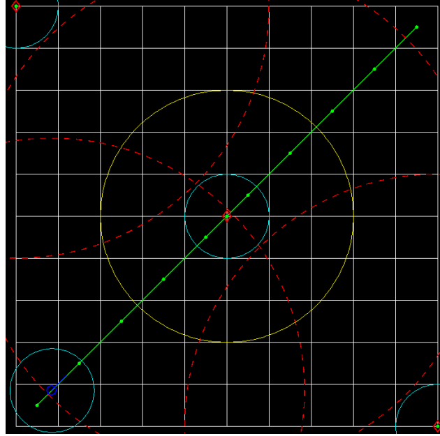
Figure 57. Initial Setup in Path Planning Example
