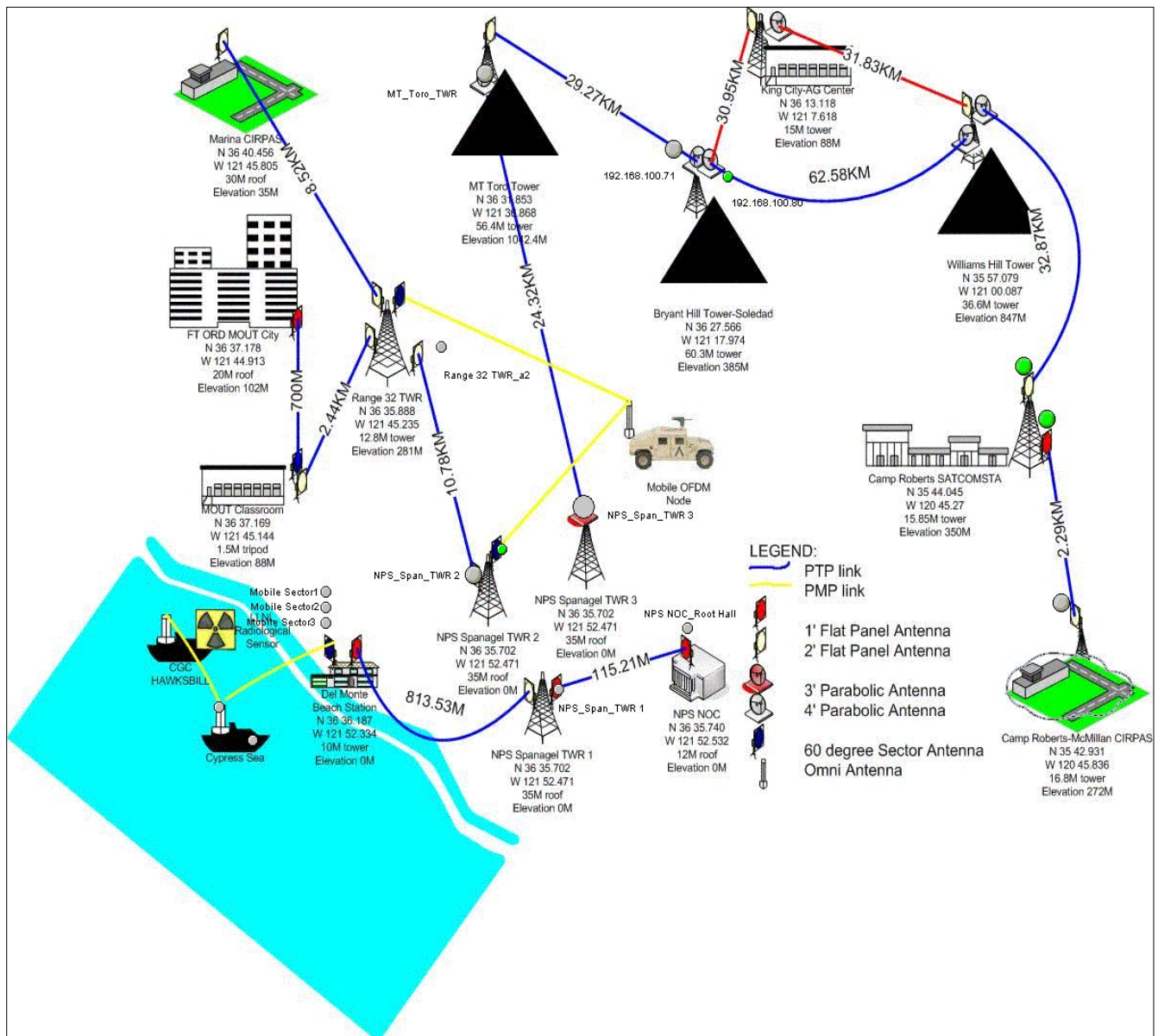
Figure 17. Experimental Network
