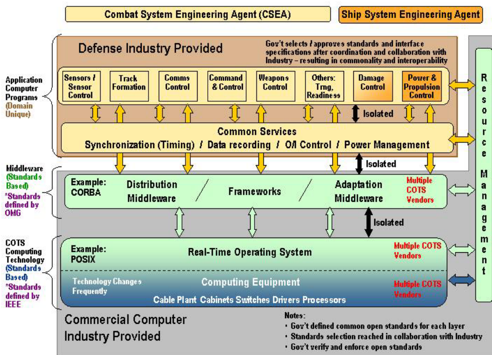
Figure 2: Notional Open System Architecture
