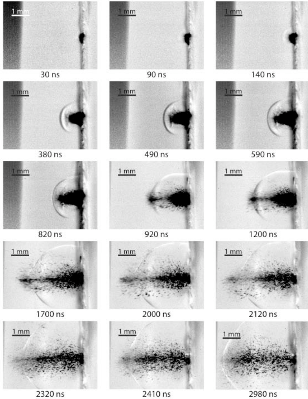
Fig. 13. Shadowgraphy images of PVN+C. The times indicate the delay of the picture to the pump laser beam. The polymer was irradiated with a fluence of 2.78 \text{ J/cm}^2 at 1064 nm.
