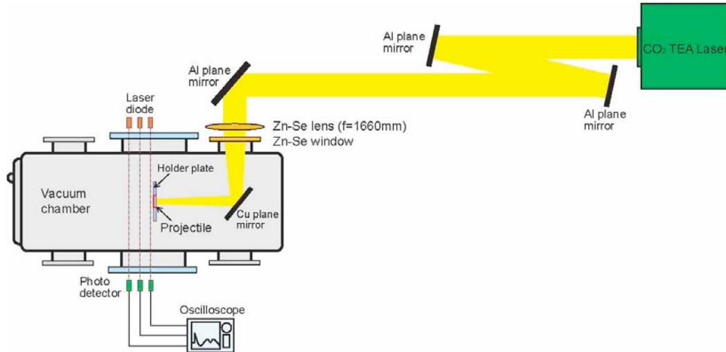
Fig. 90. Experimental Setup to measure the propagation speed of the projectile.
