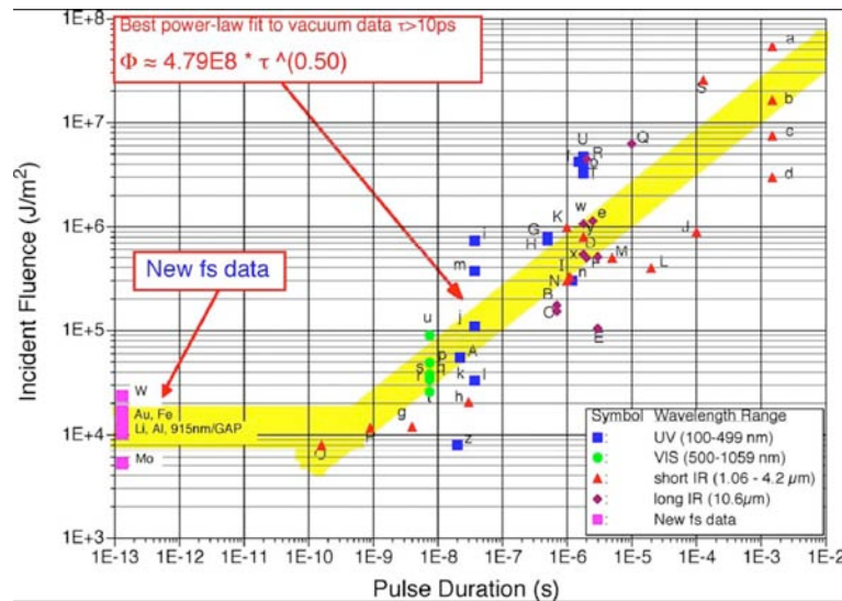
Fig. 56. Optimum coupling fluence plot shows purely thermal behavior down to 100 \text{ ps} , and a flat behavior for shorter pulses. The letters next to data points in the figure are references to the literature explained in [35]. Figure copied from [37].
