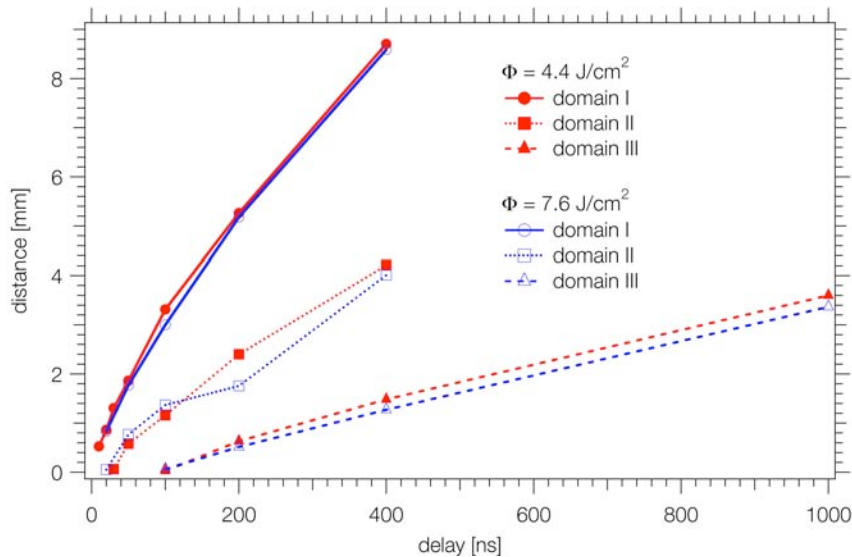
Fig. 65. The expansion of the different domains of the plasma plume of PVC+C versus the delay to the laser pulse.
