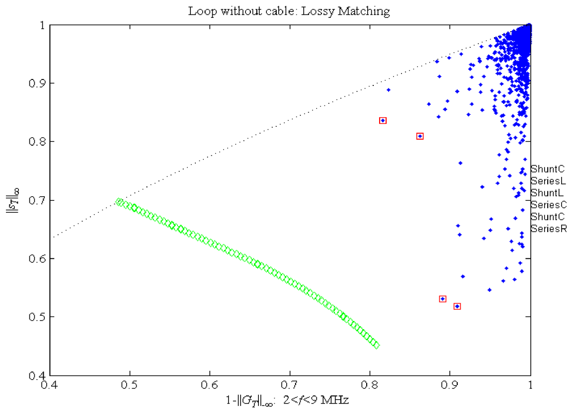
Figure 20: Gain-Reflectance for degree 5 ladder.
