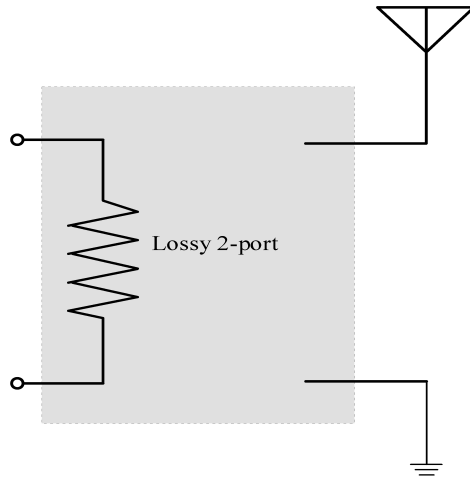
Figure 15: Perfect “matching” by a lossy 2-port.
