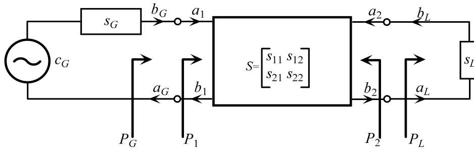
Figure 14: Reflectances and powers.
