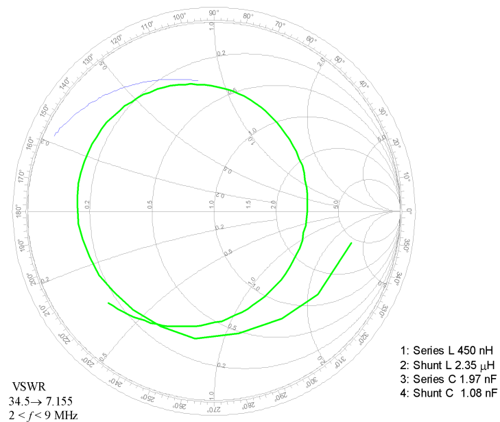
Figure 6: Matching with a general ladder of degree 4.
