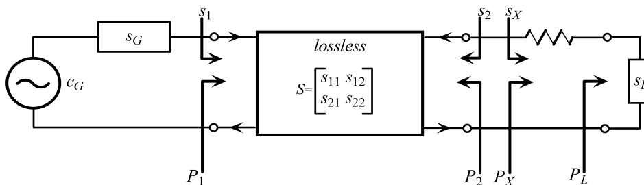
Figure 25: Lossy matching power flows.
