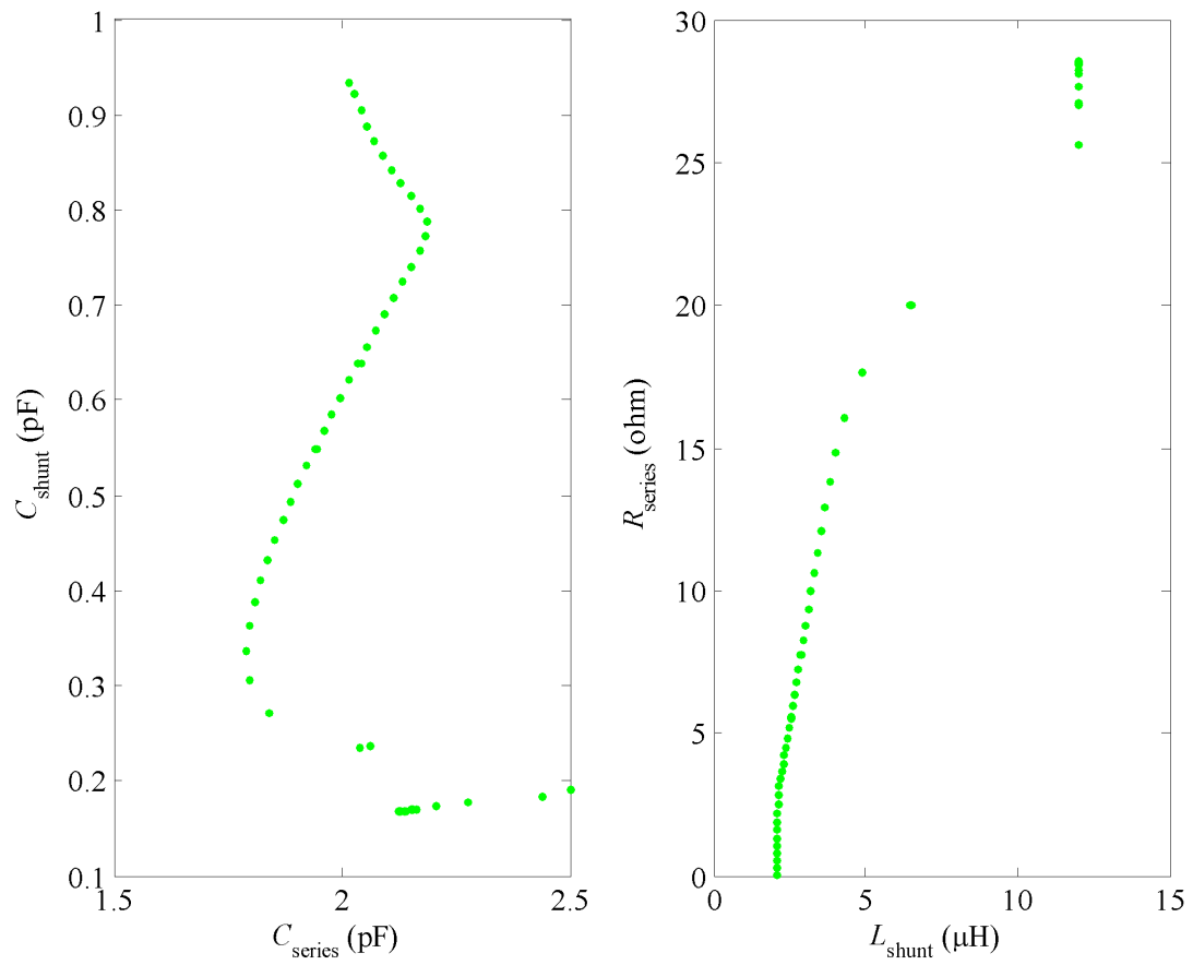
Figure 19: Pareto points.
