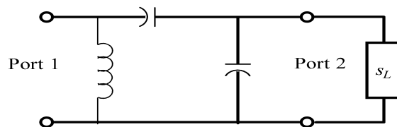
Figure 5: LC ladder n_L = 51 for degree 3.
