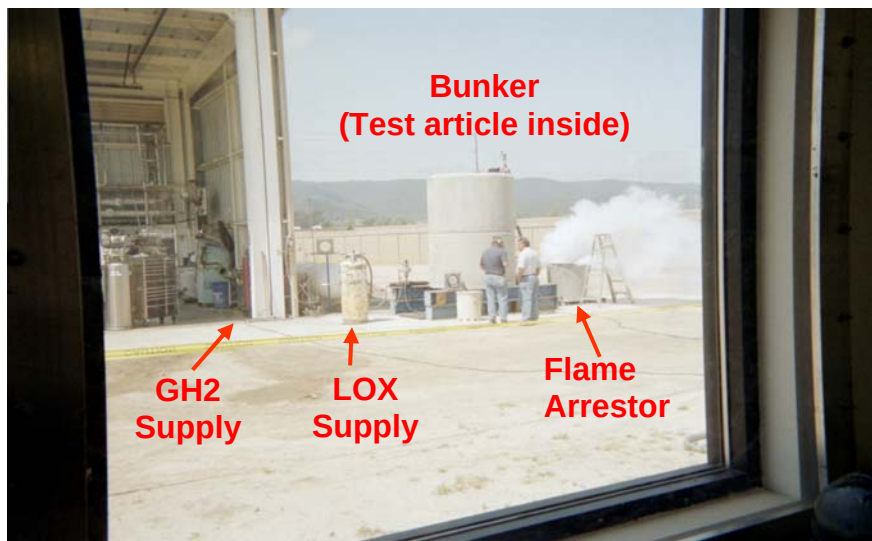
The test configuration as viewed from inside the control room. Gaseous hydrogen and LOX are supplied from tanks at left, the tank being tested is located within the bunker at center, and gases are vented at right through the flame arrestor
