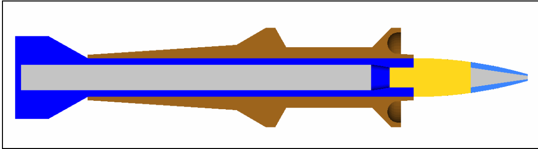
Figure 5. Case I structural configuration of the initial EAPS projectile.
