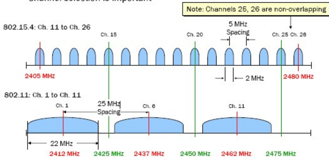
Figure 22. 802.15.4 and 802.11b Spectrum. From Ref [19].
