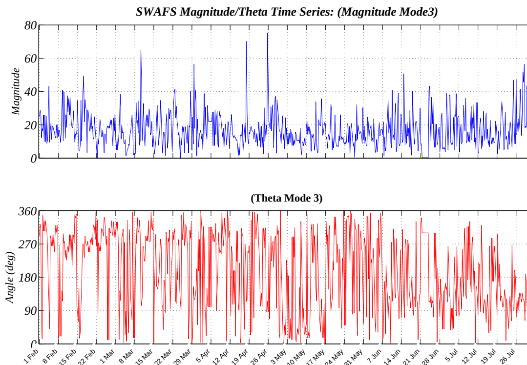
Figure 20. EOF-3 amplitude (top) and direction (bottom) for entire wind dataset in the Northern Persian Gulf.
