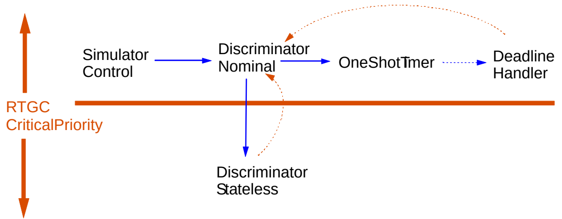
Figure 3. Collaboration diagram of the revised design
