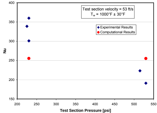
Figure 9. Effects of pressure on heat transfer for constant velocity and wall temperature. As expected, the computation as modeled is insensitive to pressure.
