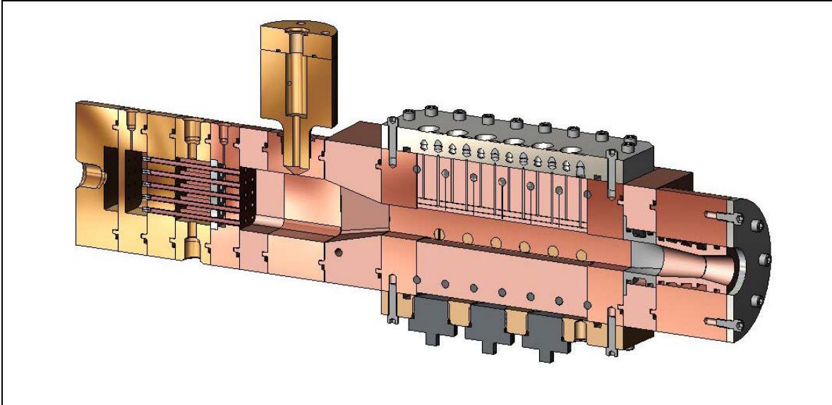
Figure 1 Heat flux test rig
