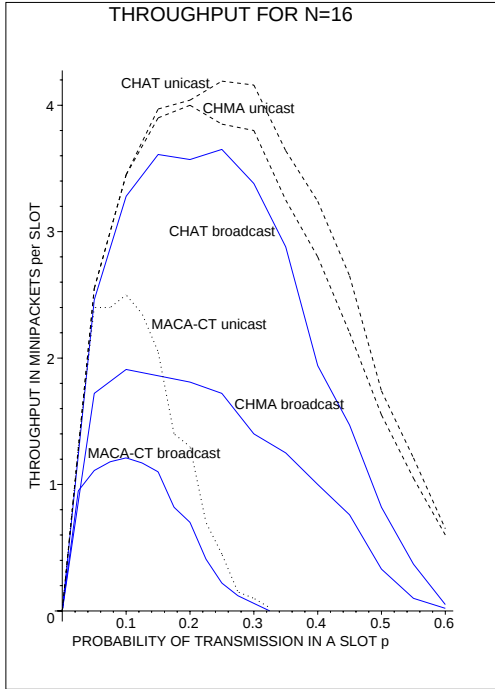
Fig. 6. Aggregate throughput for CHAT, CHMA and MACA-CT for the topology in Fig. 4(c); broadcast only traffic is compared against unicast only; the number of nodes is N = 16 and the packet length is L = 10 or approximately 150 bytes
