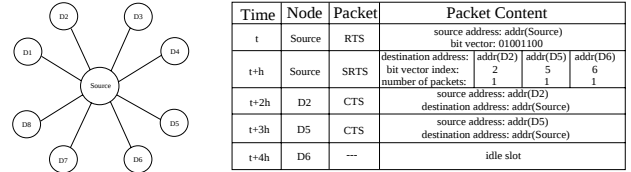
Fig. 1. Node Source transmits a data packet train to nodes D2 and D5
