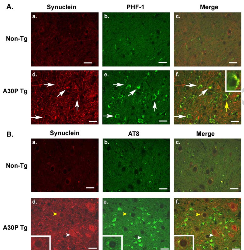
Fig. 3. Phosphorylated tau and \alpha -synuclein aggregates can occur independently. (A) Immunocytochemical analysis of \alpha -synuclein and PHF-1 immunoreactivity in the ventral pons. Staining of ventral pons from an aged nontransgenic mouse showed little \alpha -synuclein (a, c) or PHF-1 (b, c) reactivity. In contrast staining of a symptomatic A30P, transgenic mouse showed an increase in punctate \alpha -synuclein staining (d), and both diffuse and punctate staining for PHF-1 (e). Merging of the pictures shows that some of the \alpha -synuclein staining occurred in neurons containing the PHF-1 reactivity (f, arrows). Inset highlights \alpha -synuclein and PHF-1 colocalization of a single neuron (yellow arrow). Bar = 20 \mu m. (B) Immunocytochemical analysis of an aged nontransgenic mouse shows little staining of \alpha -synuclein (a, c) or AT8 (b, c). In contrast staining of a symptomatic A30P, transgenic mouse shows an increase in punctate \alpha -synuclein labeling (d), and neurons in the ventral pons with both diffuse and punctate accumulation of AT8 (e). Merging of the pictures shows that some of the \alpha -synuclein staining occurs in neurons containing the AT8 reactivity (f, arrows). Bar = 20 \mu m.
